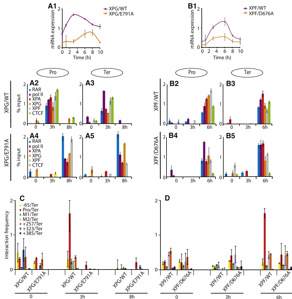
Figure 4. Endonuclease Activity of XPG and XPF Is Required for Gene Looping
