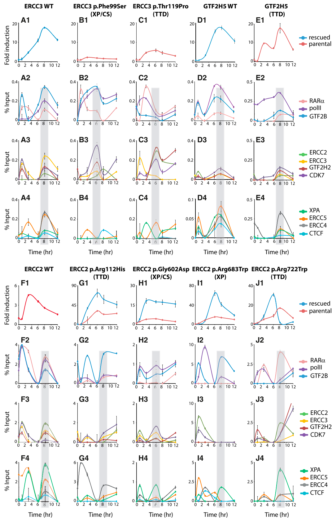
Figure 2. RARB2 mRNA Expression and Transcriptional-Machinery Recruitment on the RARB2 Promoter Are Disturbed in Cells Bearing Mutations in Genes Encoding TFIH Subunits
