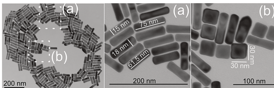
Fig. 1. TEM images of synthesized gold nanorods (GNRs). (a) and (b) show magnified views. The dimensions of the GNRs (width and length) are indicated in nm.
