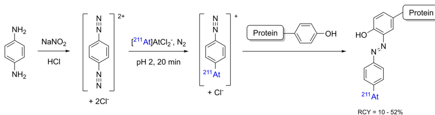
Scheme 16 211 At-labelling by nucleophilic astatodediazotation
