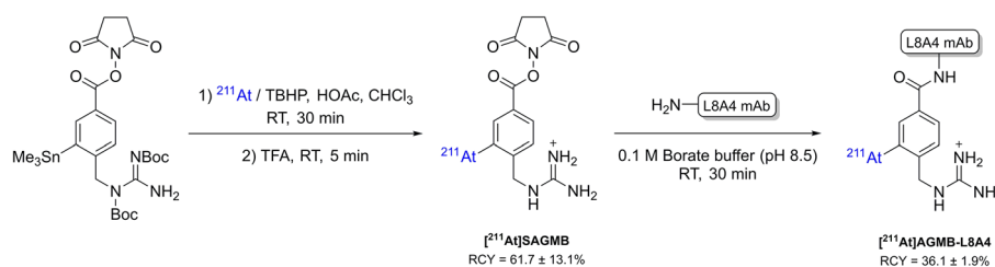
Scheme 29 ^{211}\text{At} -labelling of an antibody using the ^{211}\text{At} ]SAGMB prosthetic group agent
