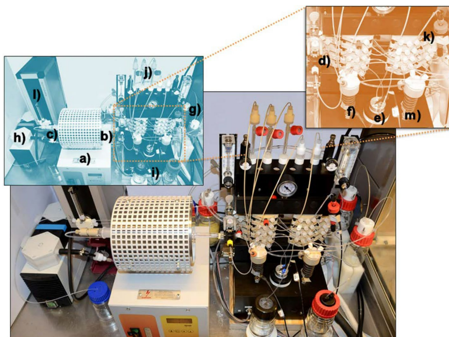
Fig. 2 Automated system for ^{211}\text{At} purification and synthesis. Reproduced from Aneheim et al. 2015a
