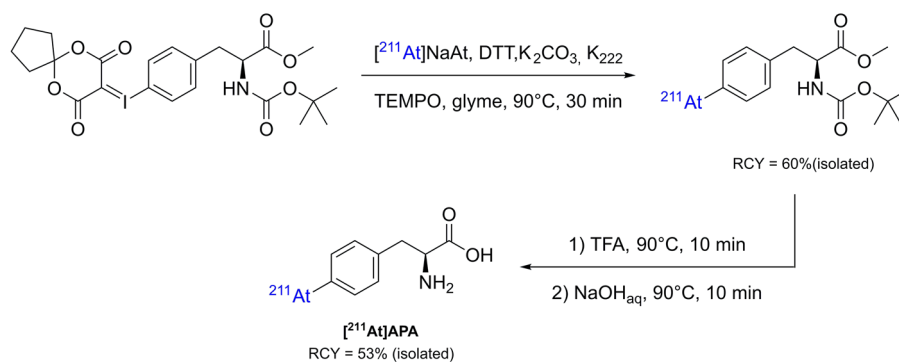
Scheme 19 211 At-labelling of aryliodonium ylides
