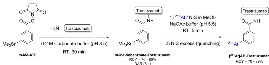
Scheme 28 Two-step and one-step procedures developed by Lindegren for the ^{211}\text{At} -labelling of antibodies via the astatobenzoyl prosthetic group
