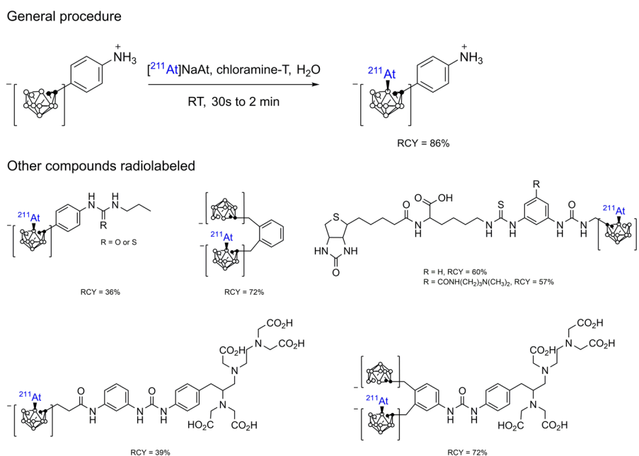
Scheme 25 ^{211}\text{At} -labelled nido-carboranyl compounds (Wilbur et al. 2004a, 2004b)
