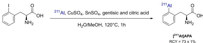
Scheme 15 ^{211}\text{At} -labelling by halogen exchange
