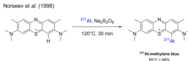
Scheme 2 Reputed examples of SEAr with ^{211}\text{At}
