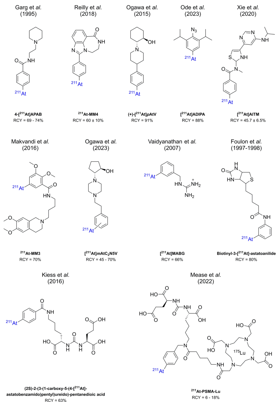
Scheme 8 Small ^{211}\text{At} -labelled molecules produced by electrophilic astatodestinylation
