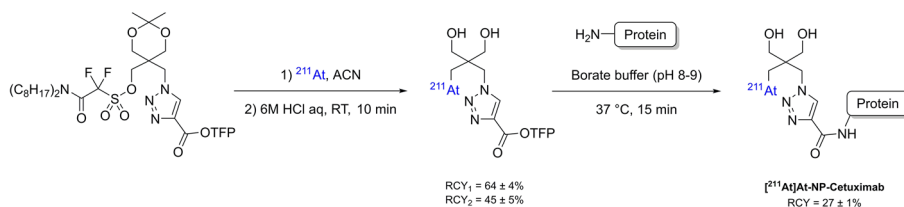
Scheme 24 ^{211}\text{At} -labelled compounds prepared using the NpG scaffold
