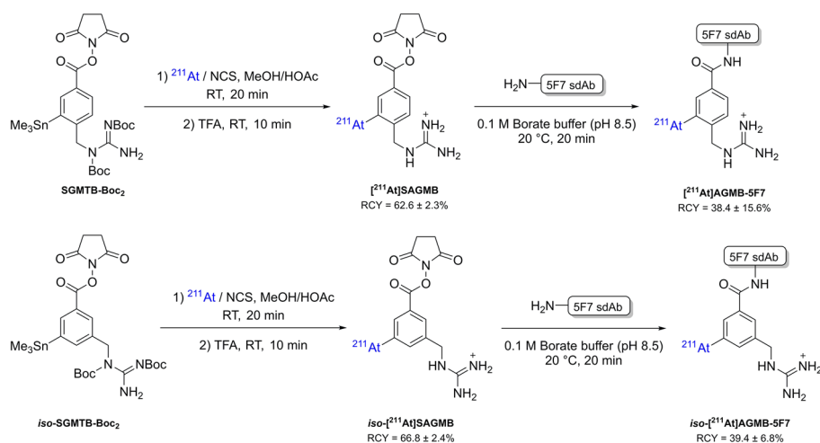
Scheme 30 Labelling of anti-HER2 single domain antibody 5F7 with ^{211}\text{At} using ^{[211}\text{At}]\text{SAGMB} or \text{iso-}^{[211}\text{At}]\text{SAGMB} . Adapted from Choi et al. (2018)
