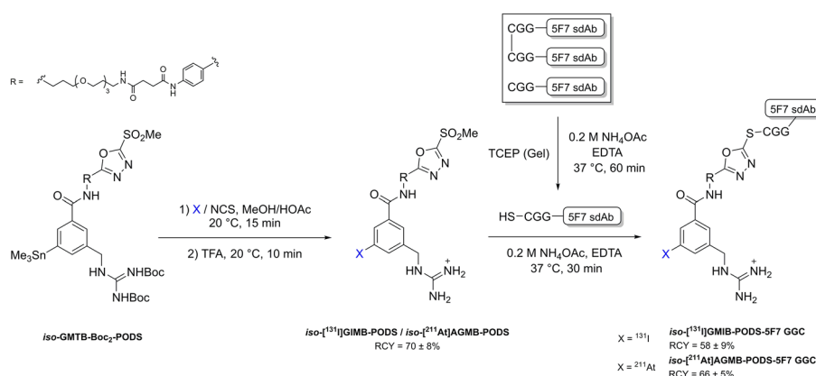
Scheme 31 Preparation of iso\text{-}[^{131}I]GMB\text{-}PODS\text{-}5F7GCG and iso\text{-}[^{211}At]AGMB\text{-}PODS\text{-}5F7GCG (Feng et al. 2022b)
