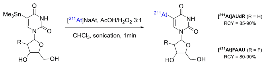
Scheme 10 Preparation of [ 211 At]AUdR and FAAU by electrophilic destannylation (Vaidyanathan and Zalutsky 1998)
