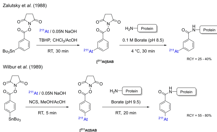
Scheme 6 Synthesis of [^{211}\text{At}]\text{SAB} by electrophilic destannylation followed by conjugation to a mAb according to Zalutsky or Wilbur
