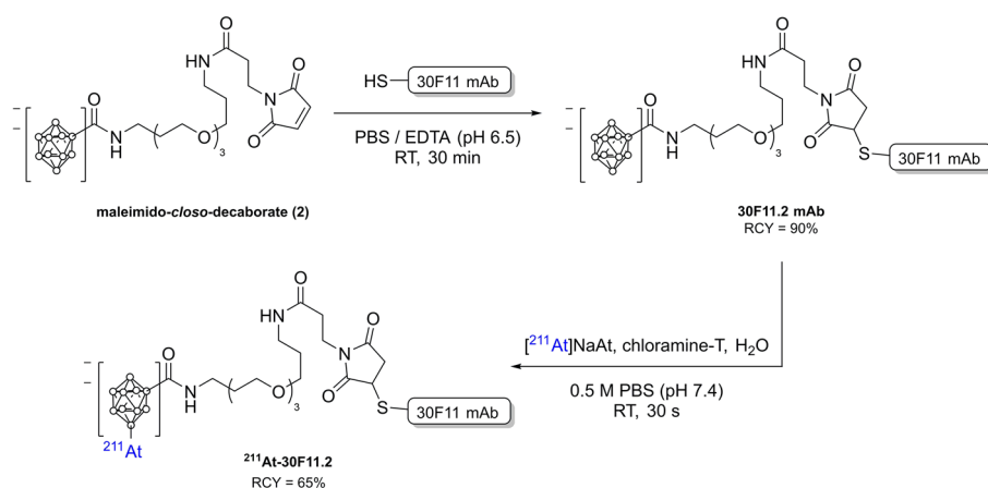
Scheme 32 Late-stage 211 At-labelling approach where sulfhydryl groups resulting from reduction of the disulphides on the mAb 30F11 are conjugated with a maleimido-closo-decaborate(2-) reagent (Wilbur et al. 2009b)
