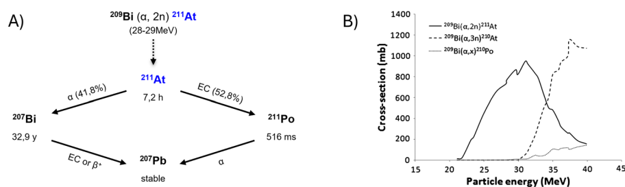
Fig. 1 A Nuclear reaction for production of ^{211}\text{At} from ^{209}\text{Bi} and decay scheme. B Cross section of the irradiation of ^{209}\text{Bi} by a particles (reproduced from Guérard et al. 2013)
