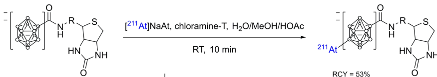
Scheme 26 ^{211}\text{At} -labelled decaborates and dodecaborates (Wilbur et al. 2007, 2009a)
