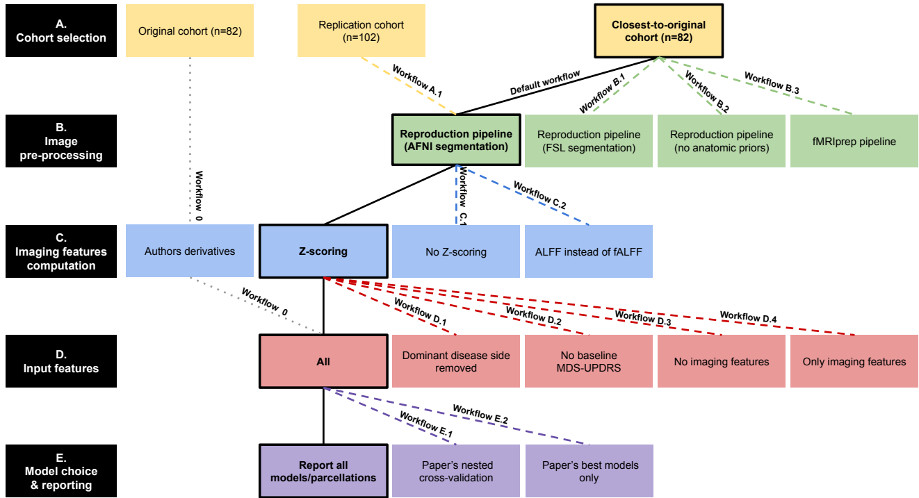
Fig 1. Summary of the different workflows implemented to reproduce and replicate the results of [1] and explore their robustness to different analytic conditions. Bold and bordered cells represent the implementation of the default replication workflow at each step, this whole workflow is labeled Default workflow and is represented using a plain bold line. The different replication workflows (Phase 1) are represented in dashed lines: all steps different from the variation follow the default workflow and each workflow corresponds to one variation from the default one. The reproduction workflow obtained with derived data provided by authors of [1] (Phase 2) is represented with a point-style line.
