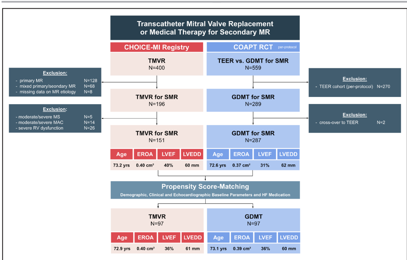
Figure 1. Study flowchart.
