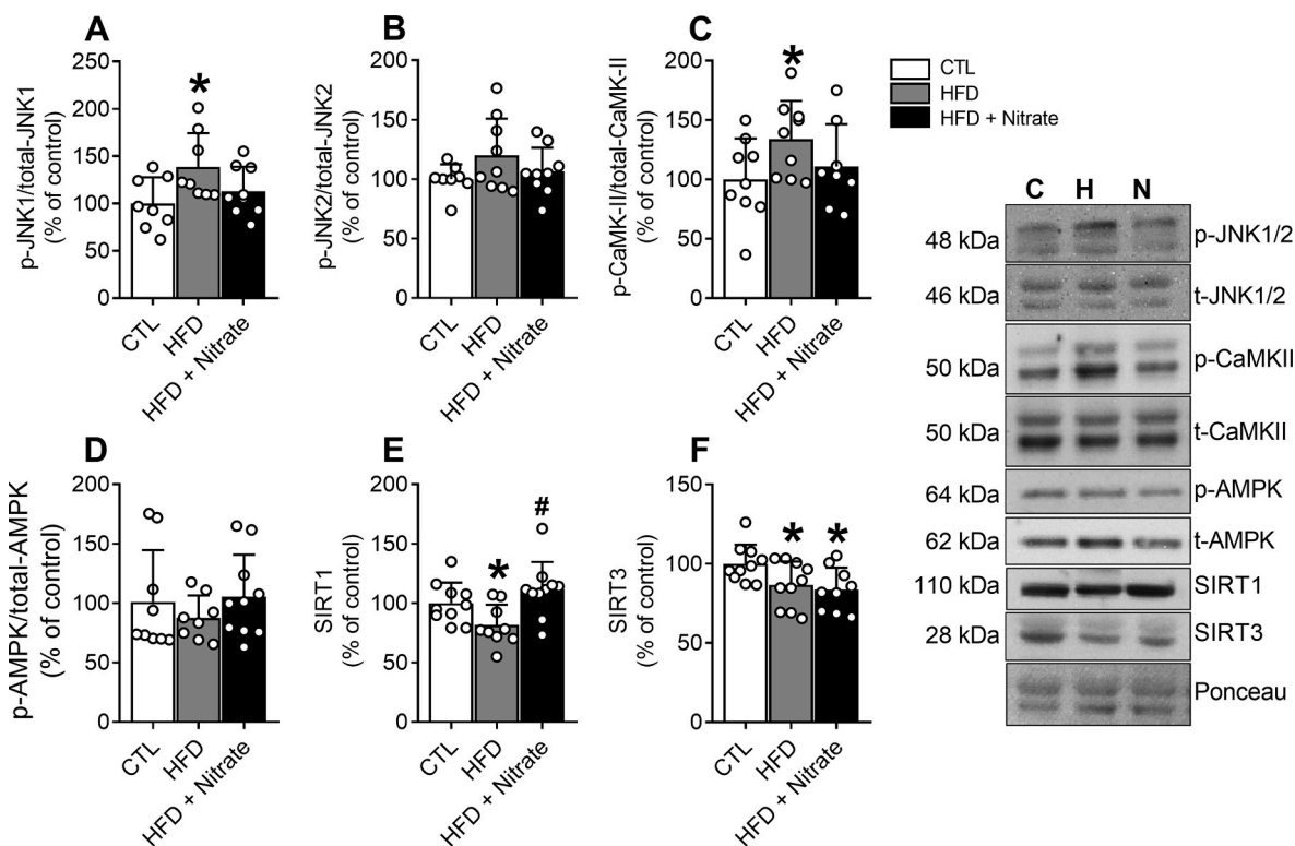
Fig. 4. – Nitrate supplementation preserves CaMK-II phosphorylation levels and rescue SIRT1 protein content. Quantification of western blotting for p-JNK1/total-JNK1 ratio (A, n = 8–9/group), p-JNK2/total-JNK2 ratio (B, n = 8–9/group), p-CaMK-II/total-CaMK-II ratio (C, n = 8–9/group), p-AMPK/total-AMPK ratio (D, n = 8–10/group), SIRT1 (E, n = 9–10/group), and SIRT3 content (F, n = 9–10/group). White bars are control-fed group, gray bars are HFD-fed group, and black bars are HFD + Nitrate group. Data are expressed with individual values and mean \pm SD superimposed. * p < 0.05 compared to control-fed group; # p < 0.05 compared to HFD-fed group. CTL – control group; HFD – high-fat diet; CaMK-II – Ca^{2+} /calmodulin-dependent protein kinase II; AMPK – AMP-activated protein kinase; SIRT1 – sirtuin 1; SIRT3 – sirtuin 3. JNK – c-Jun N-terminal. Statistical analysis: One-way ANOVA with Fisher's LSD post hoc test.
