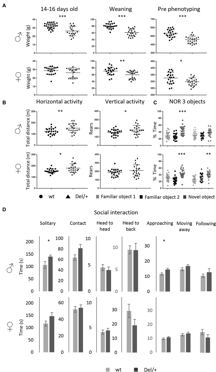
FIGURE 3 Phenotypic characterization of the 16p11.2 rat models on the LE genetic background. (A) Effects of Sult1a1-Spn deletion on body weight of LE 16p11.2 Del/+ rat model. Left: body weight (g) of the 14–16 days old males [wt ( n=27 ) and Del/+ ( n=19 )] and female rats [wt ( n=21 ) and Del/+ ( n=19 )]. Our observations showed a decreased body weight in Del/+ males compared to wt littermates [Student's t -test: t_{(44)}=3,819 ; p<0.001 ]. Central: body Weight at weaning of the males [wt ( n=21 ) and Del/+ ( n=20 )] and female rats [wt ( n=21 ) and Del/+ ( n=20 )] from LE Del/+ littermates. The deletion of the 16p11.2 region caused body weight decrease in male [Student's t -test t_{(39)}=6,550 ; p<0.001 ] and female individuals [Student's t -test t_{(39)}=3,036 ; p=0.004 ] compared to wt littermates. Right: body weight of 16p11.2 Del/+ male [wt ( n=22 ) and Del/+ ( n=20 )] and female [wt ( n=21 ) and Del/+ ( n=20 )] littermates during the first week of phenotype analysis. The male and female individuals carrying the deletion of the interest region continued to show a decrease in their body weight throughout their development [Student's t -test for males: t_{(40)}=5,550 ; p<0.001 ; Student's t -test for females: t_{(39)}=2,451 ;
