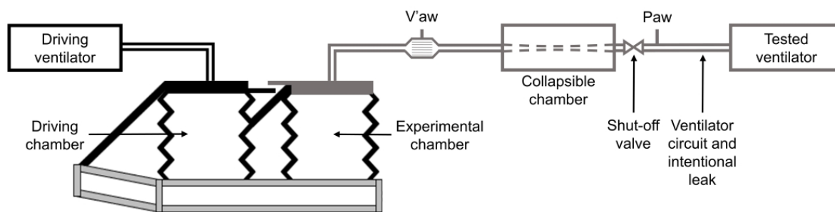
Figure 1. Experimental setup.
