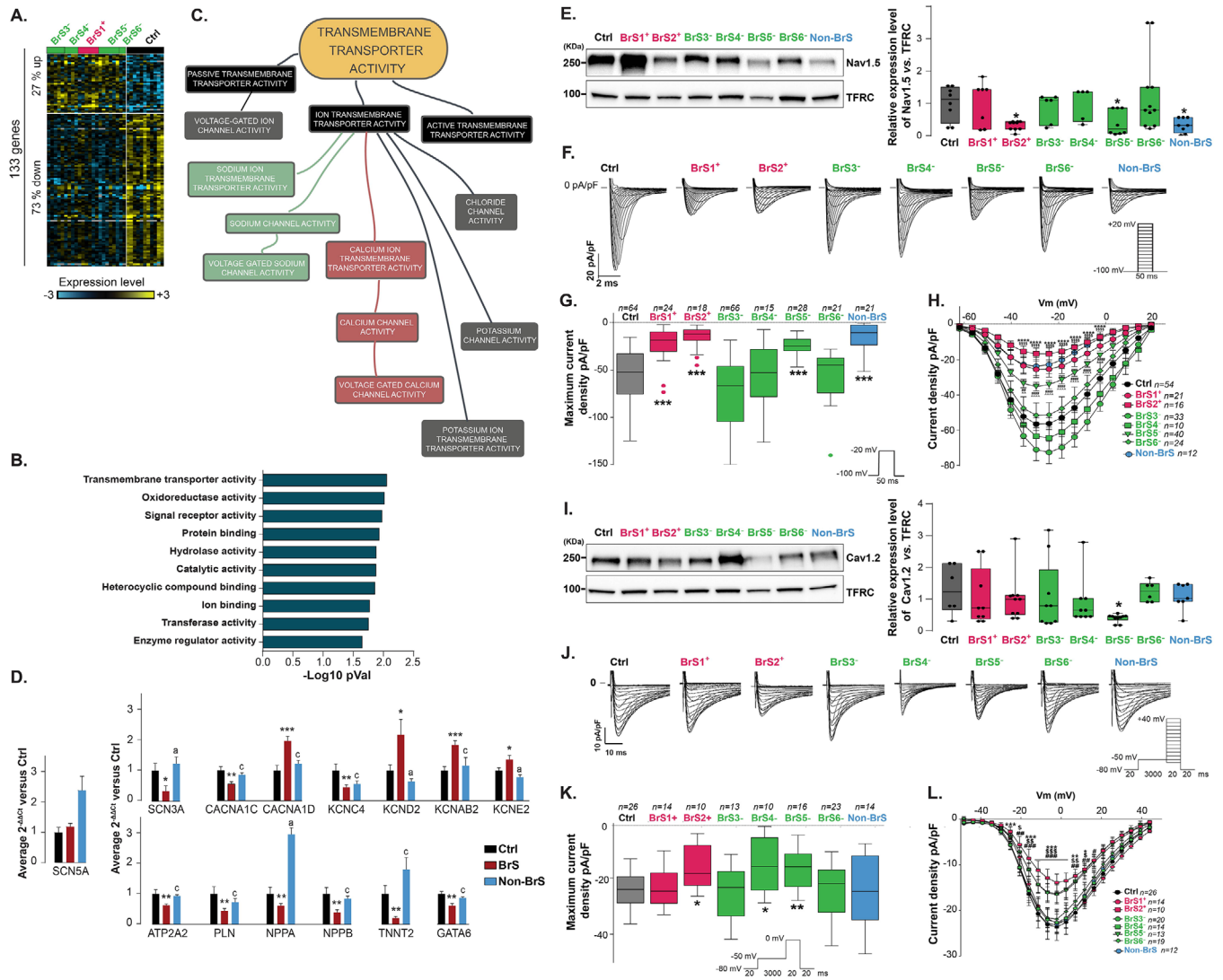
FIGURE 2 Differential gene expression profiles and variations in I_{Na} and I_{Ca,L} in BrS hiPSC-CMs as compared to controls. (A) Heatmap showing hierarchical clustering of expression profiles of 133 differentially expressed genes obtained by 3'SRP in control (Ctrl) and BrS hiPSC-CMs at day 28 of differentiation. A total of 27% were upregulated, whereas 73% genes were downregulated in BrS hiPSC-CMs. Yellow and blue represent high and low expression levels, respectively. All clones of each hiPSC line are highlighted. (B) Gene set enrichment analysis (GSEA) of gene variations obtained by 3'SRP shows gene sets with statistically altered expression patterns. (C) MindMap describing the transmembrane transporter activity alterations. (D) Expression levels of differentially expressed genes identified using high-throughput TaqMan (TLDA) in BrS hiPSC-CMs ( n = 14 ), compared to control hiPSC-CMs ( n = 12 ), and in non-BrS hiPSC-CMs ( n = 4 ) versus BrS hiPSC-CMs. p -values: *, **, and *** or a, b, and c: p < .05 , p < .01 , and p < .001 versus Ctrl or BrS, respectively ( t -test). (E) Representative immunoblots for Na_v1.5 and transferrin receptor (TFRC) in hiPSC-CMs (left panel). Ratios of Na_v1.5 expression levels (right panel, Tukey plot, n = 8 ). * p < .05 versus control (Mann-Whitney test). Na_v1.5 decreases in hiPSC-CMs from three subjects, BrS2 + and non-BrS (both carrying a stop codon in SCN5A ), as well as BrS5 - , harboring RRAD variant was observed. (F) Representative superimposed I_{Na} densities (inset: voltage-clamp protocol). Reduction was detected in BrS2 + , BrS5 - , and non-BrS, as well as in BrS1 + hiPSC-CMs carrying the N1722D- SCN5A rare variant. (G) Peak I_{Na} densities measured in control (Ctrl), BrS, and the non-affected carrier of SCN5A mutation (non-BrS) hiPSC-CMs determined at -20 mV (Tukey plot). *** p < .001 versus control (Mann-Whitney test). (H) Mean peak I_{Na} densities (pA/pF) versus membrane potential ( V_m ) recorded in hiPSC-CMs. ****, $$$$, #####, and ~~~~ p < .0001 versus control for BrS1 + , BrS2 + , BrS5 - , and non-BrS, respectively (two-way ANOVA with Bonferroni post hoc test). (I) Representative immunoblots for Ca_v1.2 , the main pore-forming subunit of the cardiac L-type calcium channel, and transferrin receptor (TFRC) in hiPSC-CMs (left panel). Ratios of Ca_v1.2 expression levels (right panel, Tukey plot, n = 8 ). A decrease in Ca_v1.2 expression was solely observed in BrS5 - hiPSC-CMs, carrying an RRAD -variant. * p < .05 versus control (Mann-Whitney test). (J) Representative superimposed I_{Ca,L} densities (inset: voltage protocol). (K) Peak I_{Ca,L} densities measured in control (Ctrl), BrS, and the nonaffected carrier of SCN5A mutation (non-BrS) hiPSC-CMs determined at 0 mV (Tukey plot). A decrease in I_{Ca,L} was observed in BrS2 + , BrS4 - and, consistently with a previous description, in BrS5 - . * p < .05 and ** p < .01 versus control (Mann-Whitney test). (L) Mean peak I_{Ca,L} densities (pA/pF) versus membrane potential ( V_m ) recorded in hiPSC-CMs. *, #, and $ p < .05 , **, ##, and $$ p < .01 , and ***, ###, and $$$ p < .001 versus control for BrS1 + , BrS4 - , and BrS5 - , respectively (two-way ANOVA with Bonferroni post hoc test)
