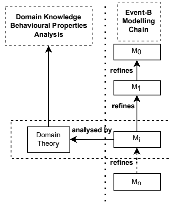
Fig. 1: Methodology overview
