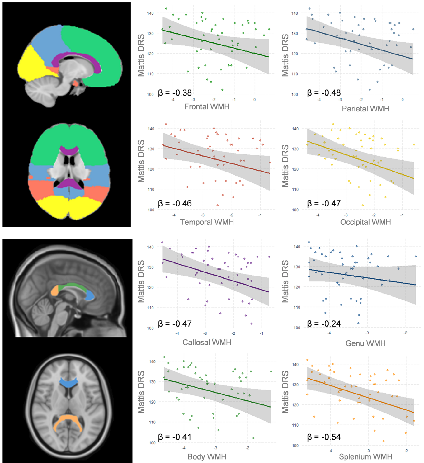
FIGURE 2 Associations between global cognition and regional white matter hyperintensities (WMH) in amyloid beta-positive Alzheimer's disease ( A\beta pos-AD). Association between regional WMH and global cognition ( Mattis Dementia Rating Scale [DRS]). Plots represent global cognition regressed onto regional WMH (total intracranial volume-corrected and log-transformed), controlling for age, sex, level of education (with 95% confidence intervals). Standardized betas ( \beta ) were added. For the sake of illustration one outlier ( Mattis-DRS = 84/144) was removed from the figure (results were unchanged with or without the outlier). Anatomic atlases were represented on the left panel for illustration purposes (Hammers atlas for lobes at the top and JHU atlas for CC at the bottom)
