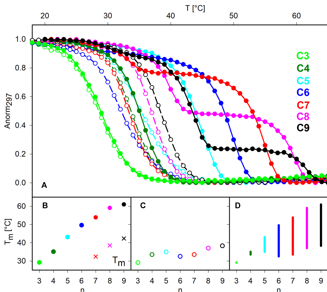
Figure 3. (A) Normalized melting (full circles) and refolding (open circles) profiles of studied C n sequences monitored by absorption at 297 nm at pH 6.5, measured with the 0.25°C/min rate of temperature change. (B) Apparent melting temperatures of the more stable (circles) and the less stable (crosses) iM species, (C) T_{ren} , and (D) hysteresis ( \Delta T = T_m - T_{ren} ) plotted against the number ( n ) of cytosines in blocks. The numerical values (average of three measurements) are in Supplementary Table S1.
