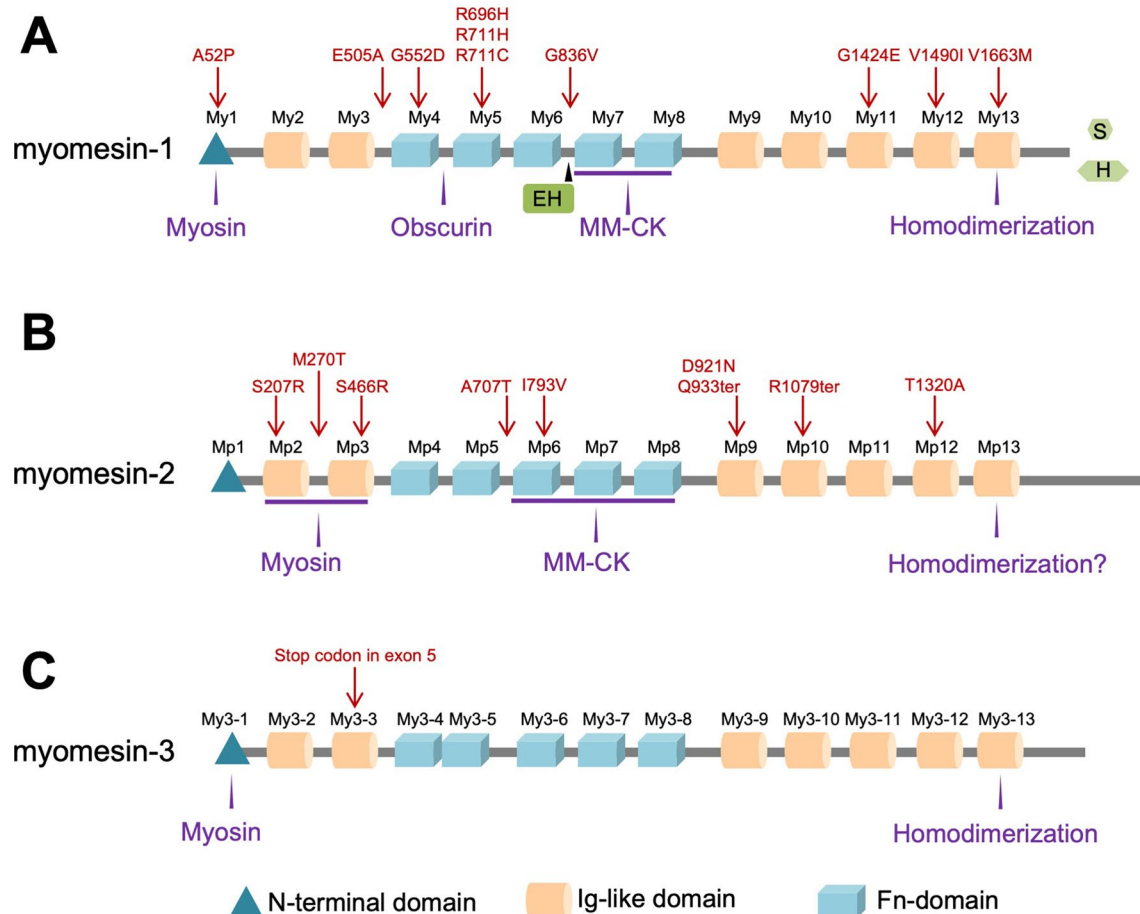
Fig. 2 Domain layout of the myomesin proteins. A myomesin-1, EH-insertion, S and H splicing variants are shown in green B myomesin-2 C myomesin-3. Interacting partners are shown in purple, variants reported in Table 1 are shown in red above their approximate position in each molecule
