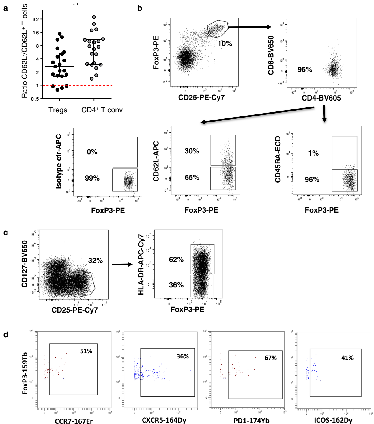
Fig. 2 Phenotype of Tregs in NSCLC. a Ratio of non-TLS to TLS CD3 + CD25 bright FoxP3 bright Tregs and CD4 + Tconv was determined according to the differential expression of CD62L ( n = 21 patients). Data are represented by median with interquartile range. Wilcoxon–Mann–Whitney U test; **P = 0.0079 . b, c Characterization of CD3 + CD25 bright FoxP3 bright cells according to CD4, CD8, CD62L, CD45RA, CD127, HLA-DR, and CD45ra expression by flow cytometry on fresh NSCLC tumors. d Illustration of the expression of CCR7, CXCR5, PD-1, and ICOS on CD3 + CD4 + CD8 - FoxP3 bright CD25 bright CD127 - CD62L + TLS-Tregs.
