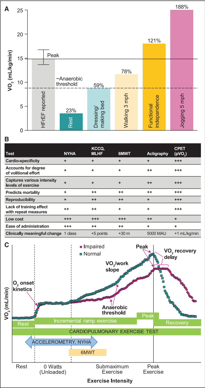
Figure 1. Functional capacity assessments. A , Oxygen uptake ( \text{VO}_2 ) required for activities of daily living relative to average \text{VO}_2 observed in 42 heart failure with reduced ejection fraction (HFrEF) trials in which peak \text{VO}_2 ( \text{pVO}_2 ) was measured. B , Comparison between commonly used assessments of functional capacity in heart failure (HF) clinical trials. C , Relative exercise intensity levels associated with measures of functional capacity in patients with HF. 6MWT indicates 6-minute walk test; CPET, cardiopulmonary exercise testing; KCCQ, Kansas City Cardiomyopathy Questionnaire; MAU, mean accelerometer unit; MLHF, Minnesota Living With Heart Failure Questionnaire; and NYHA, New York Heart Association.
