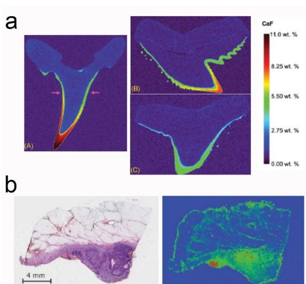
Figure 9: LIBS molecular imaging of shark teeth and LIBS elemental imaging in human skin tissues embedded in paraffin.
