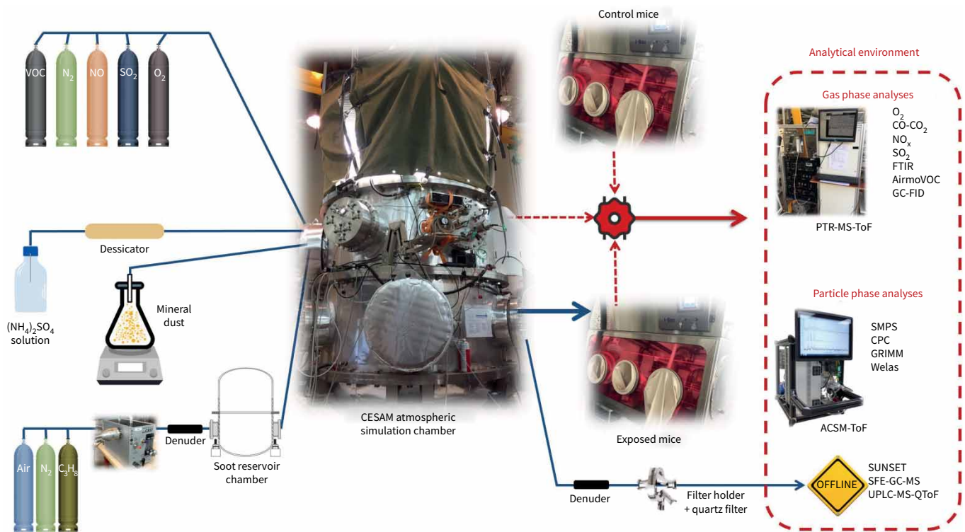
FIGURE 2 A schematic view of the atmospheric simulation, starting to the left with a continuous introduction of air and precursors in the atmospheric simulation chamber, then under the irradiation of Xe lamps at the top of the chamber the chemistry takes place, leading after a few hours to a secondary atmosphere “feeding” the exposure device where the exposed pre-clinical models are positioned, while the reference pre-clinical samples are exposed to a reference atmosphere (air filtered from pollutants). Analytical instruments allow to qualify/quantify the pollutants present in the simulated atmosphere, both online and offline (PolluRisk platform, France). ACSM-ToF: time-of-flight aerosol chemical speciation monitor; CESAM: multiphase atmospheric experimental simulation chamber; CPC: condensation particle counter; FTIR: Fourier-transform infrared spectroscopy; GC-FID: gas chromatography–flame ionisation detection; PTR-MS-ToF: proton transfer reaction time of flight mass spectrometry; SFE-GC-MS: supercritical fluid extraction with gas chromatography–mass spectrometry; SMPS: scanning mobility particle sizer; UPLC-MS-QToF: ultra-performance liquid chromatography quadrupole time of flight mass spectrometry; VOC: volatile organic compound.
