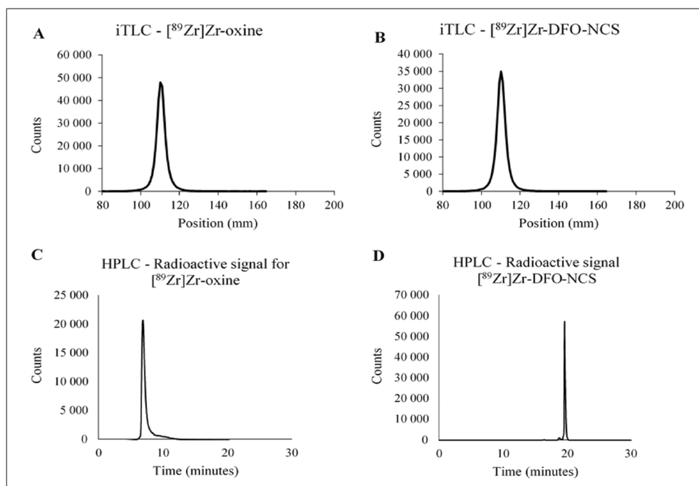
Fig. 4. Radiochemical conversion (RCC) >98 % with instant thin-layer chromatography (iTLC) for A [ ^{89}\text{Zr} ]Zr-oxine and B [ ^{89}\text{Zr} ]Zr-DFO-NCS synthesis. Radio-HPLC showing the C radioactive peak for [ ^{89}\text{Zr} ]Zr-oxine and the D radioactive peak for [ ^{89}\text{Zr} ]Zr-DFO-NCS.
