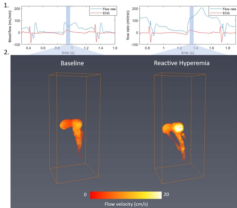
Figure 4. Coronary flow at baseline (left) and during reactive hyperemia (right). Absolute flow velocity mapping using 3D UDCA at early diastole.
