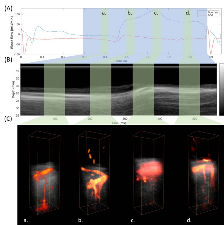
Figure 2. 3D Coronary flow imaging during diastole. (A) Phasic coronary artery blood flow measured by the coronary flow probe placed on the LAD. The blue area shows the ultrafast acquisition temporal window. The green areas show the time position of power Doppler reconstructions at late systole (a) early diastole (b) mid diastole (c) and late diastole (d). (B) Time-motion (TM) profile at the center of the imaged volume. The acquisition covers the end of the systolic phase and the entire diastolic phase. (C) 3D Power Doppler: Venous flow are mostly shown at phase (a), whereas arterial flows are shown at phase (b). During the myocardial relaxation the power Doppler was not correctly reconstructed because of the rapid tissue motion (c). Arterial flows are then reconstructed at the end of the diastole (d).
