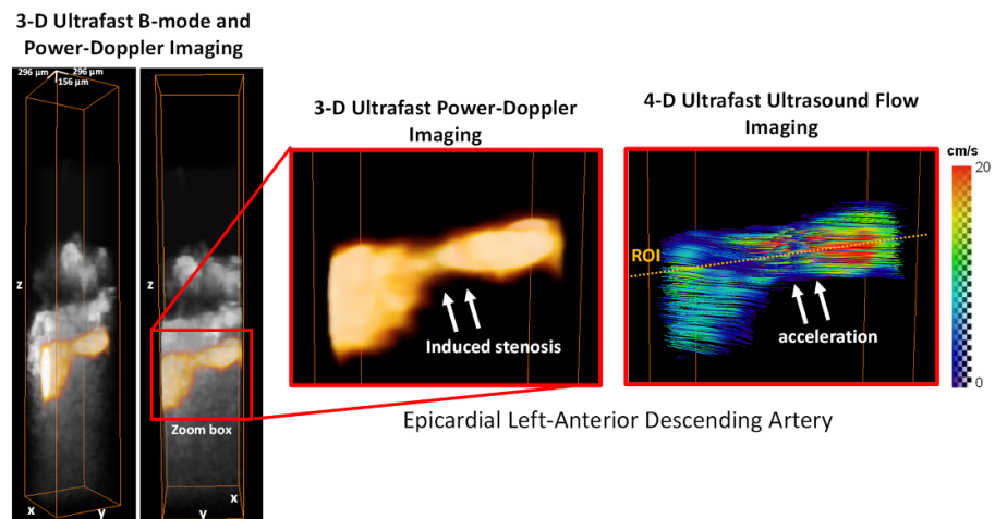
Figure 5. Epicardial LAD stenosis. Power-Doppler volumes overlaid on anatomical B-mode volumes show the induced stenosis and 4D ultrafast ultrasound flow imaging show the induced flow acceleration at the center of the stenosis.
