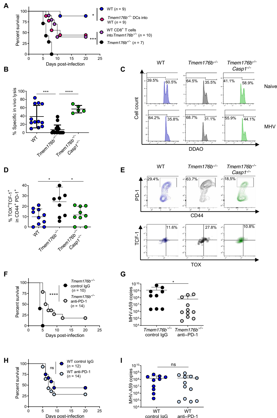
Fig. 2. Inflammasome-dependent T cell exhaustion in Tmem176b -/- mice infected with MHV-A59. (A) Survival of MHV-A59-infected WT and Tmem176b -/- mice left untreated. In another group, infected WT mice were adoptively transferred with splenic DCs from infected Tmem176b -/- animals, and Tmem176b -/- mice were adoptively transferred with CD8 + T cells from infected WT animals. * P < 0.05; *** P < 0.001, log-rank (Mantel-Cox) test. (B) Percentage of MHV-A59-specific CD8-dependent in vivo lysis was calculated with the formula described in Materials and Methods. Twelve WT, 16 Tmem176b -/- , and 5 Tmem176b -/- Casp1 -/- mice were studied at 5 dpi. *** P < 0.001; **** P < 0.0001, one-way ANOVA test. (C) Representative histograms of the experiments shown in (B). (D) Percentage of liver-infiltrating TOX + TCF-1 + within PD-1 + CD44 + cells, gated in CD8 + MHV-A59-specific T cells. Animals from two independent experiments were analyzed. * P < 0.05, one-way ANOVA test. (E) Representative dot plots of the animals analyzed in (D). (F) Survival of Tmem176b -/- mice infected with MHV-A59 and treated with control IgG or anti-PD-1 antibody. **** P < 0.0001, log-rank (Mantel-Cox) test. (G) Viral load in the liver at 5 dpi with MHV-A59 in Tmem176b -/- mice treated with control IgG or anti-PD-1 antibodies. * P < 0.05, Mann-Whitney test. (H) Survival of WT mice infected with MHV-A59 and treated with control IgG or anti-PD-1 antibody. ns, nonsignificant. Log-rank (Mantel-Cox) test. (I) Viral load in the liver at 5 dpi with MHV-A59 in WT mice treated with control IgG or anti-PD-1 antibodies. Mann-Whitney test.
