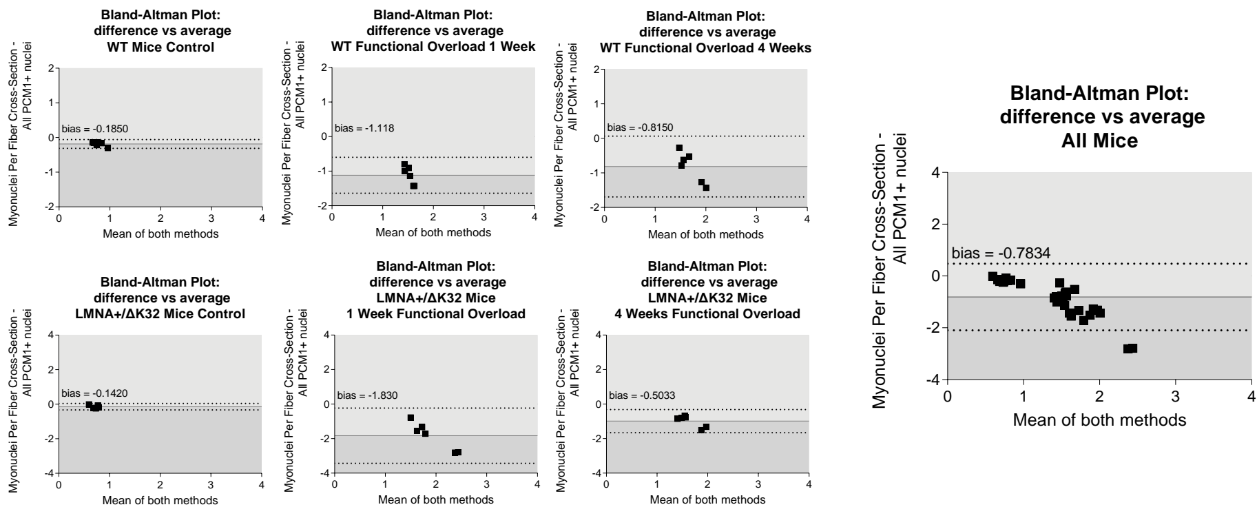
Supplementary Figure 2: Bland-Altman plot analysis comparing myonuclei per fiber cross-section measurements to manual quantification of all PCM1+ nuclei for WT & LMNA +/- ΔK32 control mice and after functional overload.
