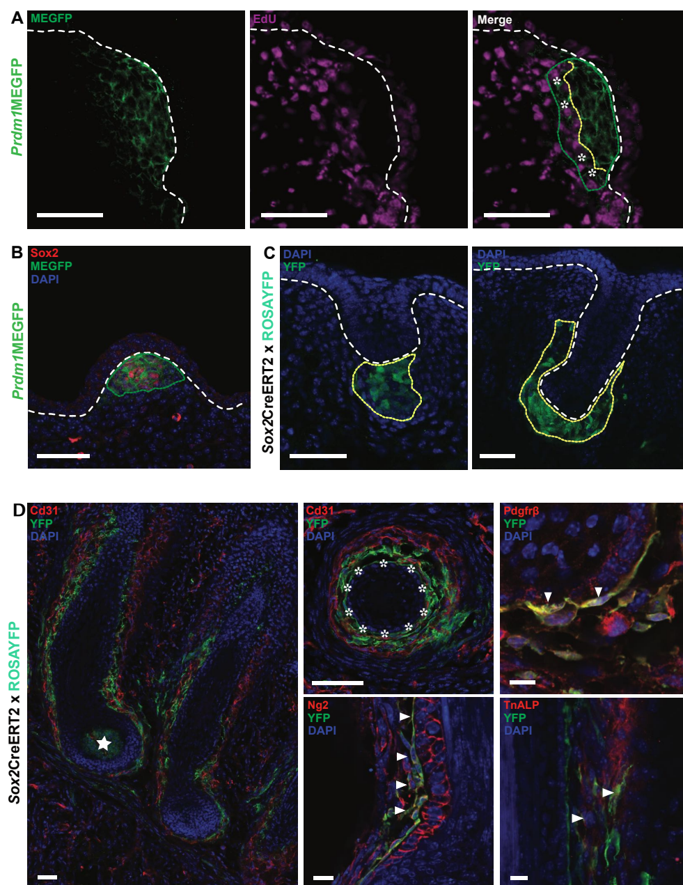
Figure 3. Prdm1/Sox2 cells in early whisker mesenchymal condensate contribute to several lineages of the adult whisker. (A) The vast majority of GFP-positive cells do not incorporate EdU, in contrast to the peripheral ones at E12.5. The yellow dashed area indicates the separation between the two populations (asterisk indicates Prdm1 + peripheral cycling cells). (B) The Sox2 immunofluorescence on Prdm1 MEGFP whisker pads reveals that Sox2 marks a subpopulation of Prdm1 positive cells. Note that Sox2 is also expressed in the putative oligodendrocytes surrounding the nerve endings surrounding the whisker pre-mesenchymal condensate. Cre expression was induced upon tamoxifen injection in E12.5 Sox2 CreERT2 crossed with ROSAYFP embryos and examined for YFP expression either in the early stages (E13, E14) or at the completion of development (E17, P3). (C) Note that YFP is first expressed in a cluster of mesenchymal cells right underneath the hair germ; when the latter becomes the hair peg, the YFP cluster envelops it into a mesenchymal cup. (D) Analysis at later time points (E17–P3) reveals the extensive contribution of YFP+ cells to several lineages of the whisker follicle including the DP (starred) and the DS (asterisks). Several YFP+ cells in close contact with the
