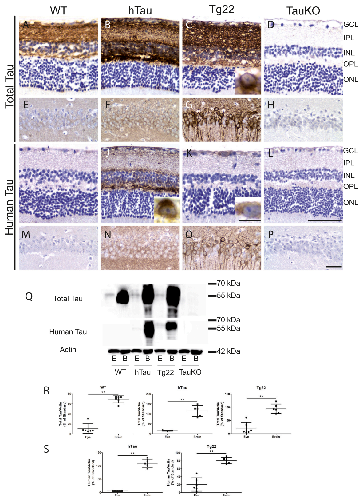
Fig. 1. Localization and expression of tau proteins in the retina of different mouse models.
