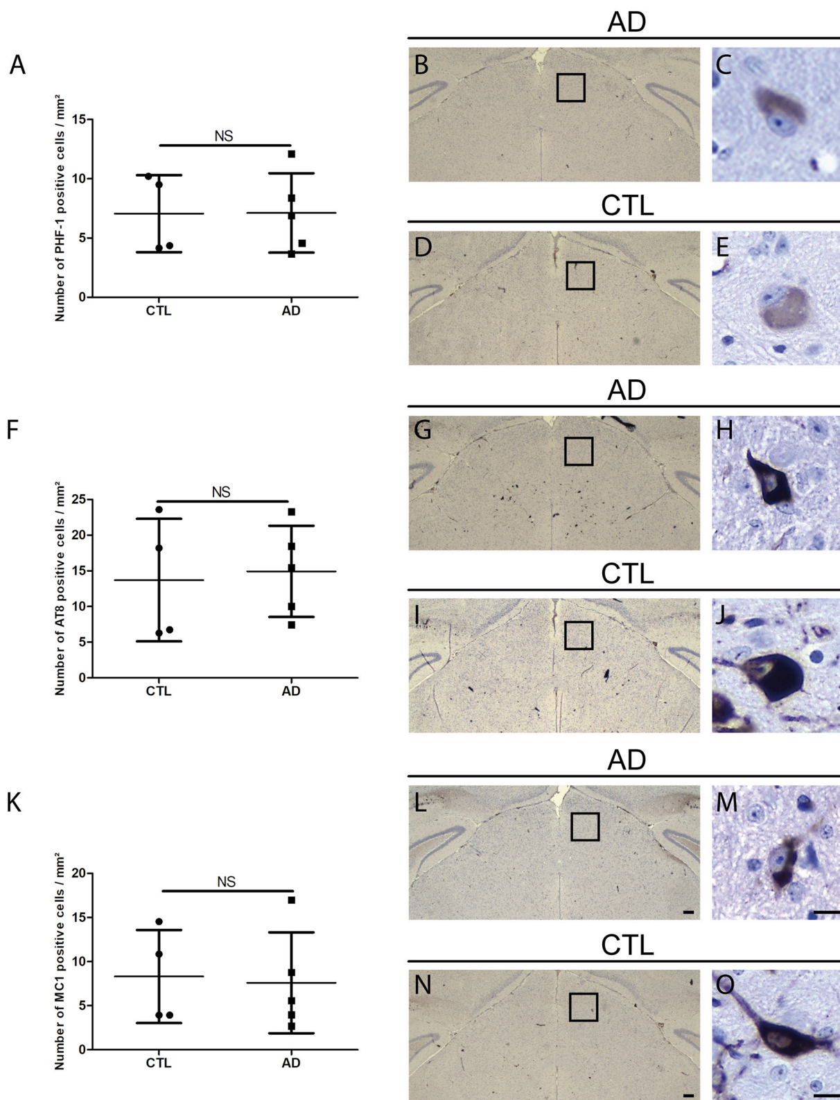
Fig. 6. Analysis of tau pathology spreading in the superior colliculus.
