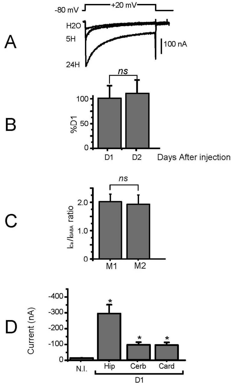
Figure 2. Expression of voltage-gated Ca^{2+} channels after injection of membrane preparation. (A) Typical current traces recorded on oocytes injected with water ( H_2O ), or hippocampal membrane preparation in response to depolarizations to +20 mV from a holding potential of -80 mV, 5 h (5 H) or 24 h (24 H) after injection. The recording medium contained 40 mM Ba^{2+} . (B) Expression was at its maximum level one day after injection (D1, set at 100%), and the current amplitude was similar at day 2 (D2) following membrane injection. (C) Histogram showing the ratio of the level of Ca^{2+} channel expression (measured as the peak current amplitude recorded during a depolarizing pulse to +10 mV in BANT40) on GABA receptor expression (measured as the peak current amplitude in response to 1 mM GABA at HP of -80 mV in ND86) for two different mice, M1 and M2. (D) Different membrane preparations (at 5 mg/mL) produced different levels of voltage-gated Ca^{2+} channel expression (N.I.: non-injected oocytes, or oocytes injected with Hip: hippocampal membrane, Cerb: cerebellum membrane or Card: cardiac ventricular membrane). ns means—not significant, *—with injection.
