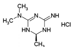
FIGURE 1 Chemical structure of Imeglimin hydrochloride salt
