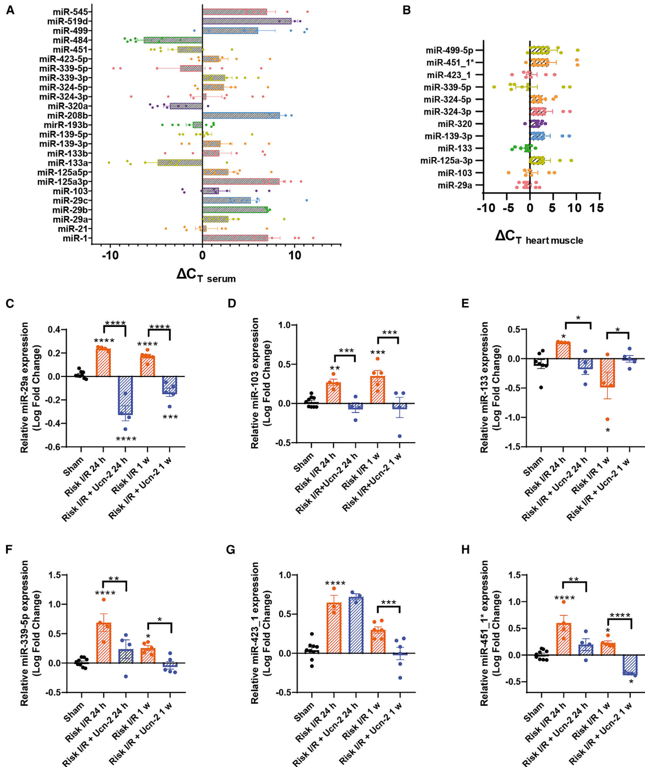
Figure 4. miRNAs expression in serum and heart tissue of STEMI patients, and in rat cardiac ventricle risk zone
