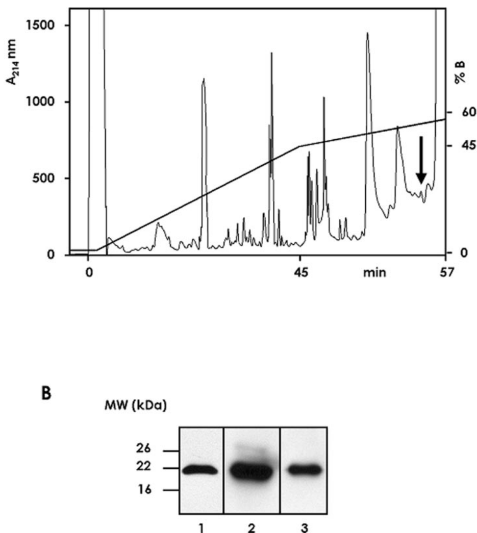
FIG. 6. HPLC purification and Western blot analysis of PEBP in bovine serum. A , 400 \mu l of serum was purified on a Macherey-Nagel reverse-phase Nucleosil 300-5 C18 column (4 \times 250 mm). Absorbance was monitored at 214 nm, and elution was performed at a flow rate of 700 \mu l/min with the gradient as indicated on the chromatogram. The arrow indicates the fraction in which PEBP was detected. B , Western blot analysis using anti-PEBP antibody was performed on a serum fraction eluted from HPLC. Lane 1 , 0.1 \mu g of PEBP purified from bovine brain; lane 2 , 10 \mu g of intragranular proteins from bovine chromaffin granules; lane 3 , serum HPLC fraction (1/4) indicated by the arrow in A . The immunoreactive band at 21 kDa corresponds to whole PEBP.
