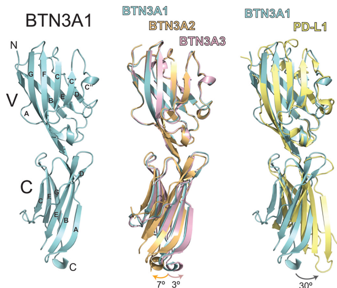
FIGURE 1. Crystal structures of the BTN3A isoforms. The structure of BTN3A1 is shown colored in cyan in ribbon format ( left panel ). BTN3A molecules are composed of a membrane-distal Ig-V domain and a membrane-proximal Ig-C domain. The canonical Ig \beta -strand designations (A–G) are shown for both. The middle panel shows superposition of the BTN3A1 (cyan), BTN3A2 (orange), and BTN3A3 (pink) structures determined in this study. The three structures are superimposed via their highly conserved V domain, demonstrating subtle shifts in the orientation of the C domain. The angle of rotation is shown at the bottom of the structures, with color-coded arrows corresponding to the particular isoform. The right panel shows structural comparison of BTN3A1 with PD-L1, the closest structural homologue to the BTN3A molecules. PD-L1 is shown in yellow. The two molecules were superimposed via their V domains, revealing a C domain shift of ~30° between the two molecules.
