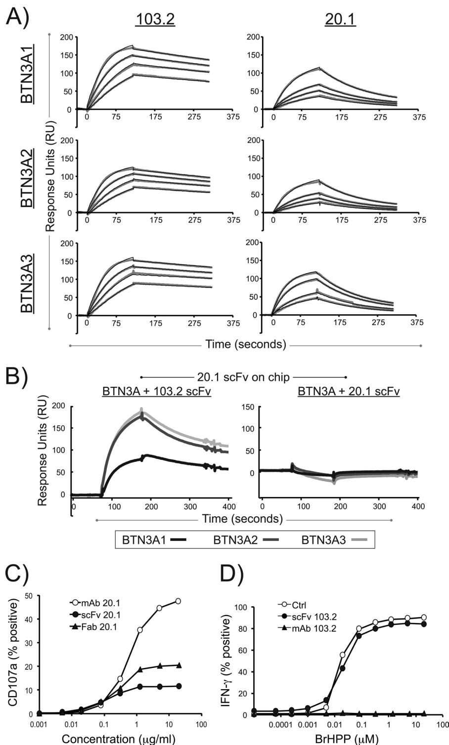
FIGURE 4. Surface plasmon resonance of the 20.1 and 103.2 antibodies with BTN3A1, BTN3A2, and BTN3A3 reveal high affinities and noncompetitive binding. A, representative sensograms are shown for the surface plasmon resonance analysis of 20.1 scFv and 103.2 scFv binding to the three BTN3A isoforms. Each BTN3A isoform was immobilized on an individual flow cell on a sensor chip, and the scFv were flowed as analyte at concentrations ranging from 10 to 80 nM. The data curves are shown in gray, and the modeled fit is shown as black lines. B, competition assay between the 20.1 and 103.2 scFv for BTN3A isoforms. The 20.1 scFv was immobilized on the sensor chip surface and complexes of either BTN3A-103.2scFv (left panel) or BTN3A-20.1 scFv (right panel) were flowed as analyte. Clear binding is observed with the BTN3A-103.2 scFv complex, whereas binding is blocked with the BTN3A-20.1 scFv, indicating that the two scFvs bind different epitopes on the BTN3A molecules. C, CD107a expression on the human V\gamma 9V\delta 2 T cell line GUI following incubation with either 20.1 full-length antibody (open circles), 20.1 Fab fragments (filled triangles), or 20.1 scFv (filled circles) used at the indicated concentrations. The data are presented as the percentages of CD107a+ \gamma\delta T cells and are representative of more than three experiments. D, IFN- \gamma expression in human V\gamma 9V\delta 2 T cell line GUI following activation by increasing doses of bromohydrin pyrophosphate/phosphostim (BrHPP) in the presence of the 103.2 full-length antibody (filled triangles), 103.2 scFv (filled circles), or no antibody (open circles). The data are presented as the percentages of IFN- \gamma + \gamma\delta T cells and are representative of more than three experiments.
