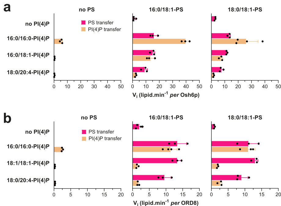
Fig. 2 Ability of Osh6p and ORD8 to transfer and exchange cellular PS and PI(4)P species. a Initial PS and PI(4)P transfer rates, measured along opposite directions, between L_A and L_B liposomes (200 \mu M total lipid each) with Osh6p (200 nM) at 30 °C, in the absence of counterligand or in a situation of lipid exchange, with diverse combinations of PS (16:0/18:1 or 18:0/18:1, 5% in L_A liposomes) and PI(4)P species (16:0/16:0, 16:0/18:1 or 18:0/20:4, 5% in L_B liposomes). Data are represented as mean \pm s.e.m. ( n = 3-4 ). b Similar experiments were conducted with ORD8 (240 nM) at 37 °C using 18:1/18:1-PI(4)P instead of 16:0/18:1-PI(4)P. Data are represented as mean \pm s.e.m. ( n = 3-4 )
