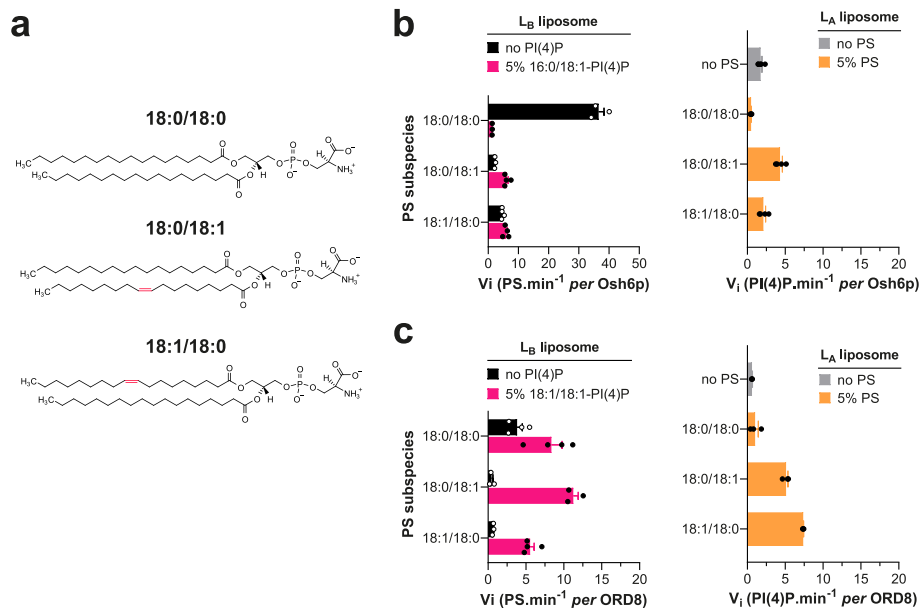
Fig. 3 Transfer of 18:1/18:0-PS vs 18:0/18:1-PS by Osh6p and ORD8. a Chemical structure of 18:1/18:0-PS compared to that of 18:0/18:0-PS and 18:0/18:1-PS. b Initial rates of PS and PI(4)P transfer, measured along opposite directions, between L_A and L_B liposomes (200 \mu M total lipid each) with Osh6p (200 nM) at 30 ^{\circ} C, in non-exchange or exchange contexts with 18:0/18:0-PS, 18:0/18:1-PS, or 18:1/18:0-PS (5% in L_A liposomes) and 16:0/18:1-PI(4)P (5% in L_B liposomes). Data are represented as mean \pm s.e.m. ( n = 3-4 ). c Similar experiments were performed with ORD8 (240 nM) at 37 ^{\circ} C using 18:1/18:1-PI(4)P instead of 16:0/18:1-PI(4)P
