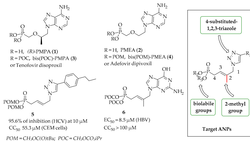
Figure 1. Structure of selected acyclic nucleoside phosphonates (ANPs) and target derivatives. PMPA: 2-(phosphonomethoxy)propyladenine; PMEA: 9-(2-(phosphonomethoxy)ethyl) adenine; POM: pivaloyloxymethyl; POC: (isopropylloxycarbonyl-oxymethyl)-ester.
