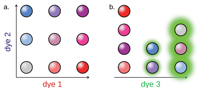
Fig. 12 Example of fluorescent particle barcoding. (a) Fluorescent particle barcoding allows to overcome the "one color per target" barrier by combining intensity levels of fluorophores. In this example, using 2 dyes, each of which can be introduced in 3 distinct intensity levels, allows the barcoding of up to 3^2 = 9 subpopulations. (b) Reporting is performed using an independent fluorescence channel, the intensity of which can be used to compute the miRNA concentration.
