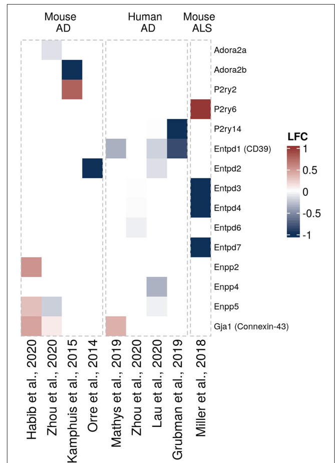
FIGURE 4 | Differentially expressed purinergic genes in astrocytes in neurodegeneration. Heatmap shows Log 2 fold changes in expression of genes involved in purinergic signaling pathways between disease (AD or ALS, or relevant mouse models) and control samples. LFC values above 1 and below -1 are shown in the same color intensity for visualization purposes. Studies were selected according to the following criteria: transcriptomic analysis was performed on single cells or nuclei and allows disease/control comparisons for selected cell types, or on bulk-sorted glial populations; differential expression analysis results were provided by authors as supplementary material and were accessible. In total, nine data sets from eight studies were included for astrocytes [Orre et al. (69) (mouse, AD model, bulk), Kamphuis et al. (70) (mouse, AD model, bulk), Miller et al. (71) (mouse, ALS model, bulk), Mathys et al. (72) (human, AD, single-nuclei), Zhou et al. (68) (two data sets, mouse AD model and human AD patients, single-nuclei), Habib et al. (73) (mouse, AD model, single-nuclei), Lau et al. (61) (human, ALS, single-nuclei), Grubman et al. (74) (human, AD, single-nuclei)] (61, 68–74).
