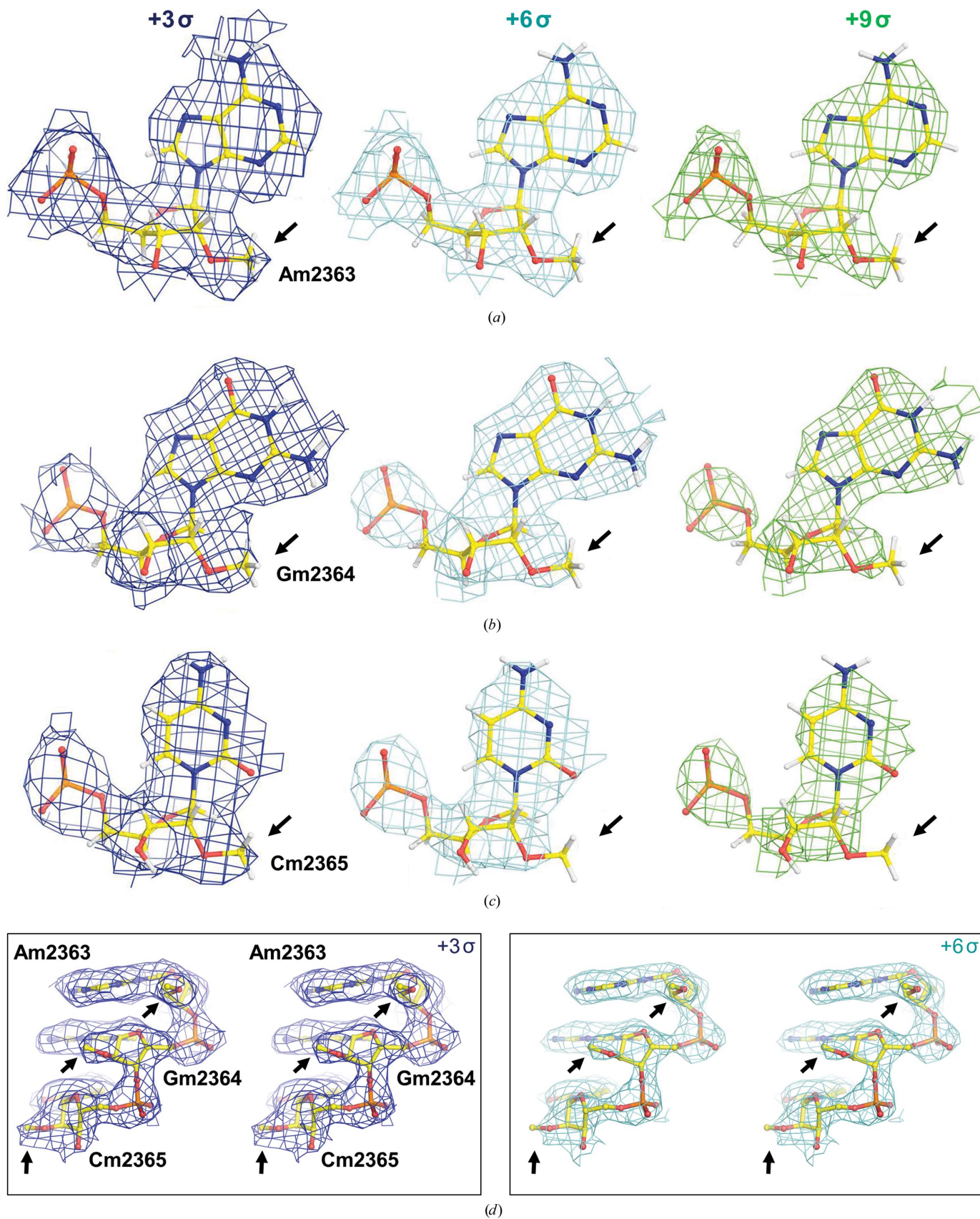
Figure 3 Quantitative comparison of three consecutive nucleotides with different levels of 2'- O -methylation. (a) Am2363 at three contour levels, (b) Gm2364, (c) Cm2365. (d) Stereo diagrams at +3σ (left) and +6σ (right) contour levels. Am2363, Gm2364 and Cm2365 have strong, medium and weak densities, respectively, suggesting differential levels of 2'- O -methylation.
