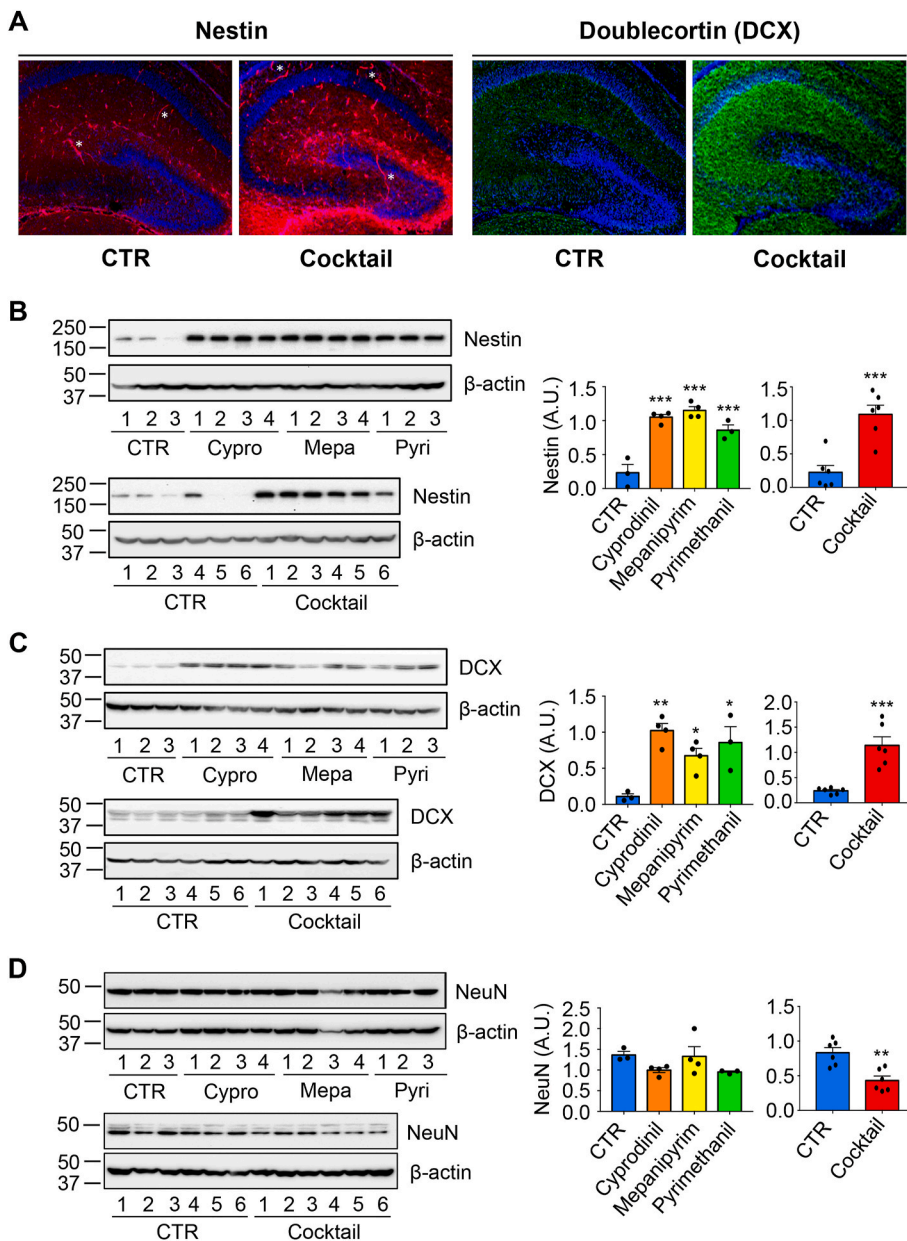
Fig. 4. In utero exposure to fungicides exacerbates the proliferation of neural precursor cells and induces a decrease of mature neurons in P3 neonates. A. Representative images of hippocampal illustrating the labelling with anti-nestin (left panel) or anti-doublecortin (DCX, right panel) antibodies of P3 neonates exposed during gestation to an equivalent volume of DMSO (CTR) or to a cocktail of the three fungicides (0.1 \mu\text{g/L} of each compound). Scale bar: 100 \mu\text{m} . White stars on the images show non-specific labelling of GFAP linked to the blood vessels. Protein levels of nestin ( B ), DCX ( C ) and neuronal nuclear antigen (NeuN, D ) were analyzed from brain homogenates of P3 mice exposed to 0.1 \mu\text{g/L} of fungicides, either alone or in cocktail. Mice treated with an equivalent volume of DMSO ( 3 \times 10^{-5}\% ) were used as controls (CTR). Protein loading was performed using an anti- \beta -actin antibody. Membranes were revealed with a Chemidoc MP imager and signals were quantified on Fiji software. All signals quantified were normalized using \beta -actin signals and results are displayed as mean \pm SEM. Statistical differences were analyzed using a one-way ANOVA followed by a Holm-Sidak's post-hoc analysis (single treatment vs CTR) or a student T-test (CTR vs Cocktail) ( \alpha = 0.05 , * p -value < 0.05 , ** p -value < 0.01 , *** p -value < 0.001 ). Black dots on graphics represent the distribution of each value obtained per animal. Numbers (1–6) correspond to brain homogenates from different animals analyzed ( n = 3 –6 animals per group). Cypro: cyprodinil, Mepa: mepanipyrim and Pyri: pyrimethanil.
