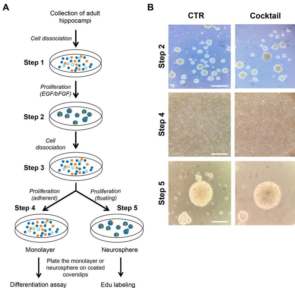
Fig. 7. Proliferation and differentiation assays of adult neural stem cells extracted from 4-months old mice exposed to a cocktail of fungicides. A. Hippocampi collected from WT mice exposed to the cocktail of fungicides or to an equivalent volume of DMSO during gestation up to 4-months old were dissociated in appropriate medium to isolate aNSC (Step 1); proliferation medium containing EGF and bFGF was used for 7–10 days until the formation of neurospheres (Step 2). Dissociation of neurospheres were done to analyze their properties using different assays (Step 3). To analyze their differentiation potential into neurons, aNSC were seeded in adherent monolayer condition (Step 4). In parallel, to analyze their proliferation properties (Edu assays), aNSC were cultivated in floating condition (Step 5). B. Representative images of aNSC isolated from CTR and fungicide cocktail exposed animals at the different steps (2, 4 and 5). Scale bars: 400 \mu\text{m} (Steps 2 and 4) and 200 \mu\text{m} (Step 5).
