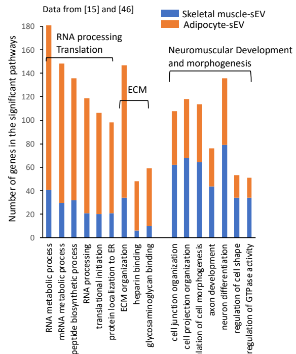
Proteins from adipocyte-sEV vs myotube-sEV
