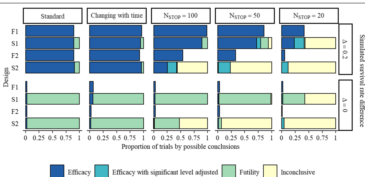
Fig. 3 Proportion of significant tests with distribution of conclusions for each design and specific case ( p_c = 0.50 ). Abbreviations: p_c indicates control survival rate; \Delta : simulated survival rate difference; F1: fixed single-arm design; S1: group-sequential single-arm design; F2: fixed two-arm design; S2: group-sequential two-arm design; “Standard”: specific case with a fixed control survival rate; “Changing with time”: specific case with an increase of the control survival rate over time; “Stopping of recruitment”: specific case with a fixed control survival rate and an early stop of the trial due to an outbreak end. For group-sequential trials, the total of trials demonstrating an efficacy of the experimental treatment was defined by the sum of trials with a significant test and trials with an adjusted p -value inferior to 0.025. The p -value was adjusted for underrunning by the method proposed by Whitehead [18]
