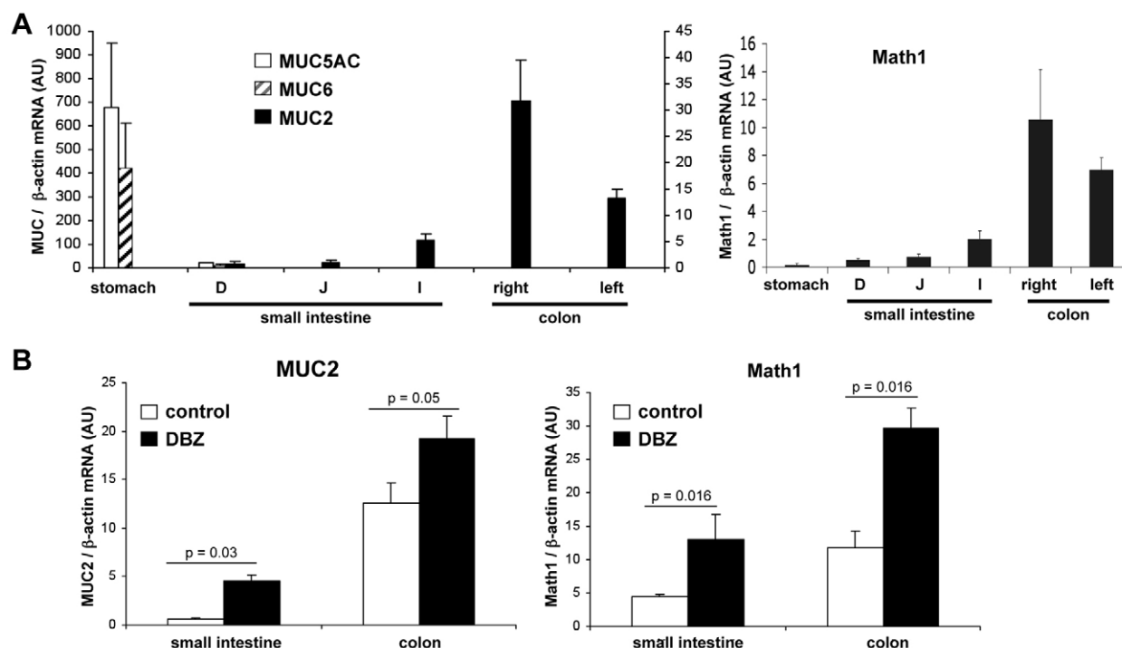
Fig. 1. Expression of various Muc and Math1 mRNAs along the entire mouse gastrointestinal tract of normal mice and mice treated with the GSI DBZ.
