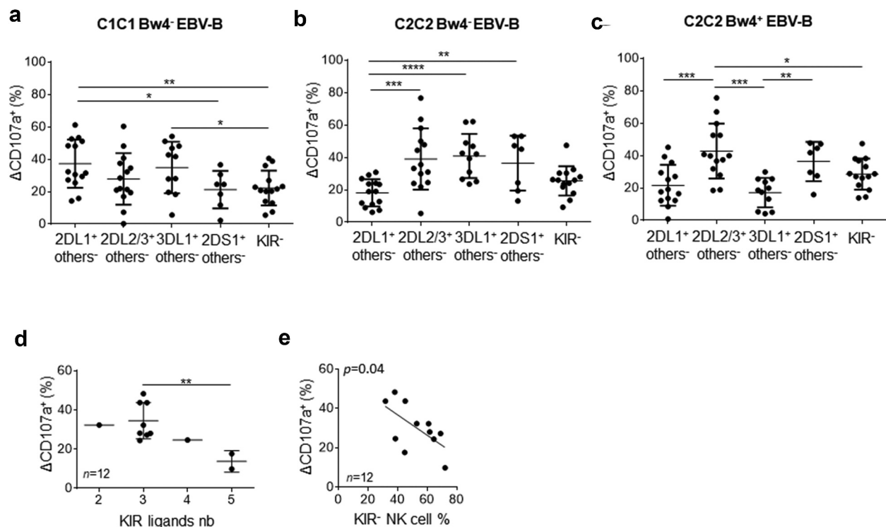
Figure 2. Lower modulator effect of KIR2DL2/3 than KIR2DL1, KIR3DL1 and KIR2DS1 on rituximab-dependent NK cell degranulation. RTX-dependent NK cell degranulation (ΔCD107a + ) frequency for each targeted NK cell subset: 2DL1 + others - , 2DL2/3 + others - , 3DL1 + others - , 2DS1 + others - and KIR - NK cells against (a) C1C1 Bw4 - EBV-B cell line, (b) C2C2 Bw4 - EBV-B cell line, and (c) C2C2 Bw4 + EBV-B cell line. ANOVA test. (d) RTX-dependent NK cell degranulation (ΔCD107a + ) frequency following KIR ligands number. The Student's t-test was performed between the series with three and five KIR ligands. (e) Correlation between percentage of RTX-dependent NK cell degranulation (ΔCD107a + ) frequency and the KIR - NK cell frequency. * p < .05 , ** p < .01 , *** p < .005 , **** p < .0001 .
