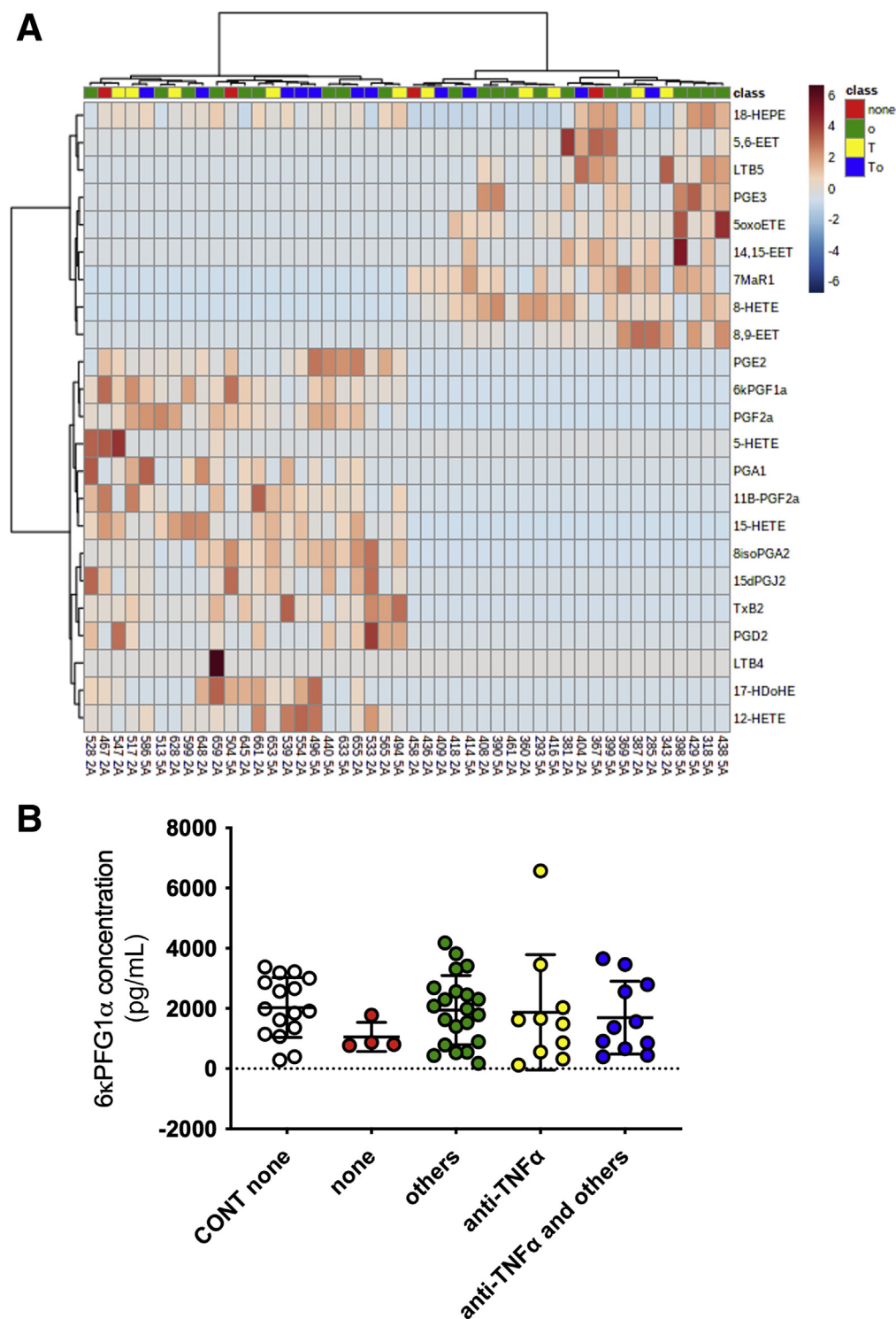
Figure 3. n -6/ n -3 PUFA-derived metabolite profiling in biopsy supernatants from IBD patients according to treatments.
