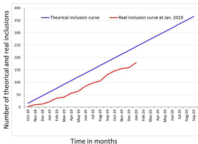
Figure 4 Theoretical and real inclusions curves. The blue curve shows the rate of expected hypothetical inclusions needed to complete recruitment on time (n=366). The red curve shows the real number of inclusions between October 2018 and January 2020 (n=178).
