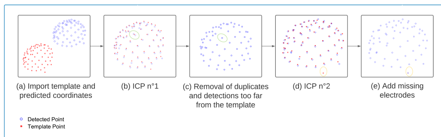
Figure 2: Description of the registration-based refinement step. (a) in blue: the prediction points from the deep learning-based step, in red: the template obtained by averaging on the training set, (b) a first ICP is performed in order to register the two points cloud, (c) for each template point, only the closest detection is kept, (d) then, a second ICP is performed and the number of detections is now less than or equal to 65, (e) finally, the points in the model not associated with any predictions are added to our final result, which therefore contains exactly 65 detections.
