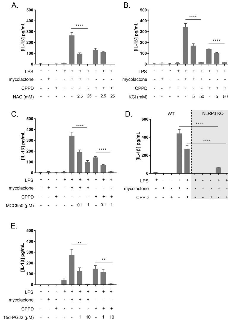
Fig 4. Mycolactone induces IL-1 \beta secretion by activating the NLRP3/1 inflammasome pathway. Three known inhibitors of the inflammasome pathway implicated in the secretion of IL-1 \beta were added to LPS-stimulated BMDM cultures in the presence of mycolactone (3 ng/mL) or CPPD (20 \mu g/mL). A. The addition of 2.5 mM or 25 mM N-acetyl-L-cysteine (NAC) decreased and totally abolished IL-1 \beta secretion, respectively, in the presence of either mycolactone or CPPD. B. The addition of 5 mM or 50 mM KCl to the medium decreased and abolished IL-1 \beta secretion, respectively, in the presence of either mycolactone or CPPD. C. The addition of MCC950, a specific inhibitor of the NLRP3 inflammasome, at a concentration of 0.1 \mu M or 1 \mu M, significantly decreased IL-1 \beta secretion in the presence of either mycolactone or CPPD. D. IL-1 \beta secretion levels were significantly lower in LPS-stimulated BMDMs with a knockout (KO) for NLRP3, in the presence of either mycolactone (3 ng/mL) or CPPD (20 \mu g/mL), than in wild-type BMDMs. E. The addition of 15-deoxy \Delta 12,14-prostaglandin J2, which inhibits both the NLRP3 and NLRP1 inflammasomes, at a concentration of 10 \mu M or 1 \mu M, decreased and abolished IL-1 \beta secretion, respectively, in the presence of either mycolactone or CPPD. Results are expressed as means + SEM of three independent experiments (triplicates of each condition in each independent experiment). Nonparametric Mann-Whitney U tests were used for the statistical analysis. P -value: * p <0.05, ** p <0.01, *** p <0.001, **** p <0.0001.
