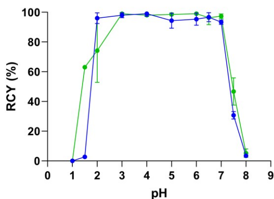
Fig. 1. Influence of pH on the ^{125}\text{I} -radioiodination (●) and ^{211}\text{At} -astatination (●) of 4-chlorobenzeneboronic acid ( 1 ). RCYs determined by radio-HPLC analysis of the crude product. Standard conditions: ( 1 ) (0.25 mM), Cu(OTf) 2 pyr 4 (10 mM), 1,10-phenanthroline (10 mM), [ ^{125}\text{I} ]NaI or [ ^{211}\text{At} ]NaAt (1-5 MBq), Tris buffer 0.5 M / DMF (85 / 15), 30 min, 100 \mu\text{L} , 23 °C, n ≥ 2.
