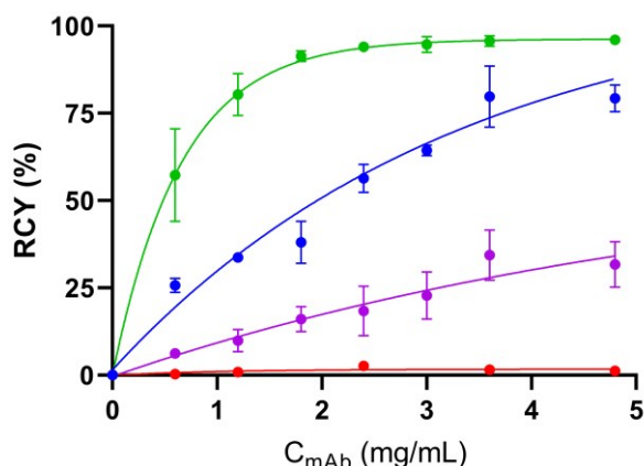
Fig. 2. Influence of mAb concentration on the ^{125}\text{I} -radioiodination a of aBA-9E7.4 (●) and 9E7.4 (●) and ^{211}\text{At} -astatination b of aBA-9E7.4 (●) and 9E7.4 (●). RCYs determined by radiolTLC-SG analysis of the crude product. Standard conditions: 30 min, 100 \mu\text{L} , 23 ^{\circ}\text{C} , Tris buffer 0.5 M pH 6 / DMF 92.5 / 7.5 n \geq 2. a \text{Cu}(\text{OTf})_2\text{pyr}_4 (5 mM), 1,10-phenanthroline (5 mM), ^{125}\text{I}]\text{NaI} (1–5 MBq) b \text{Cu}(\text{OTf})_2\text{pyr}_4 (2.5 mM), 1,10-phenanthroline (2.5 mM), ^{211}\text{At}]\text{NaAt} (1–5 MBq)
