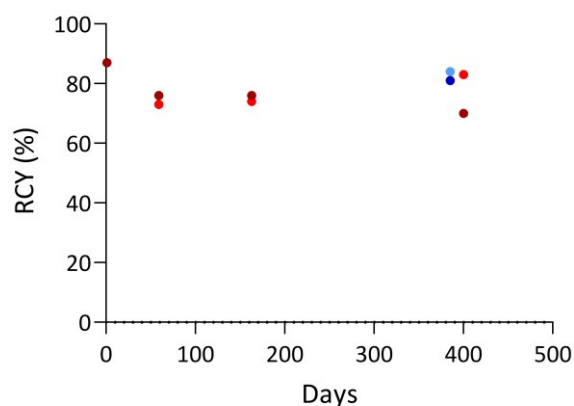
Fig. 3. Radiolabelling of aBA-9E7.4 with ^{125}\text{I} after storage at 4 °C (●) or -18 °C (○) a and ^{211}\text{At} after storage at 4 °C (●) or -18 °C (○) b in Tris buffer 0.5 M at pH 6. Standard conditions: 30 min, 100 \mu\text{L} , 23 °C. a \text{Cu}(\text{OTf})_2\text{pyr}_4 (5 mM), 1,10-phenanthroline (5 mM), ^{125}\text{I}]\text{NaI} (1–10 MBq) b \text{Cu}(\text{OTf})_2\text{pyr}_4 (2.5 mM), 1,10-phenanthroline (2.5 mM), Tris buffer 0.5 M pH 6 / DMF (92.5/7.5), ^{211}\text{At}]\text{NaAt} (1–5 MBq). RCYs determined by radioITLC-SG analysis of the crude product
