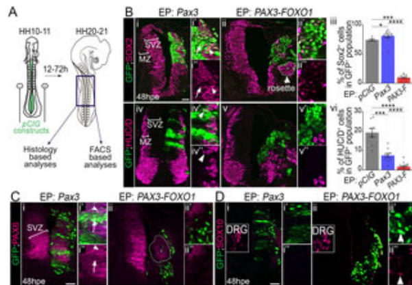
Fig 1. PAX3-FOXO1 switches off generic neurogenic marker expression in chick embryonic spinal cord. (A) Schematics showing HH10-11 chick embryos filled with pCIG based constructs before being injected into thoracic region (dark blue square) of the electroporated embryos were dissected 12 to 72 h or FACS based analyses. (B) (i-ii''; iv-v'') Immunodetection of GFP, SOX2 and HUC/D on thoracic embryos 48hpe with the indicated plasmids. MZ: Mantle Zone; SVZ: Sub-Ventricular Zone. (i-ii''; iv-v'') HUC/D + cells in the GFP + population 48hpe with the indicated plasmids (dots: embryo value; Whitney U test: *: p<0.05, ***: p<0.001, ****: p<0.0001). (C, D) Immunodetection of GFP, PAX6 and SOX10 in sections of chick embryos 48hpe with the indicated plasmids. DRG: dorsal root ganglia. Arrows: SOX10 + ; GFP + cells. x' and x'' panels are blow-ups of a subset of x panel GFP + cells. Dash lines: rosettes of GFP - cells clustering apart from the SVZ. Arrowheads in Bi', ii'' and Ci', ii'' point at a PAX6, while those in iv', iv'' point at a HUC/D + ; GFP + cell. Arrows in Bi', ii'' and Ci', ii'' mark GFP + SOX2 or PAX6. hpe: hours post-electroporation; scale bars: 50μm. https://doi.org/10.1371/journal.pgen.1009164.g001
