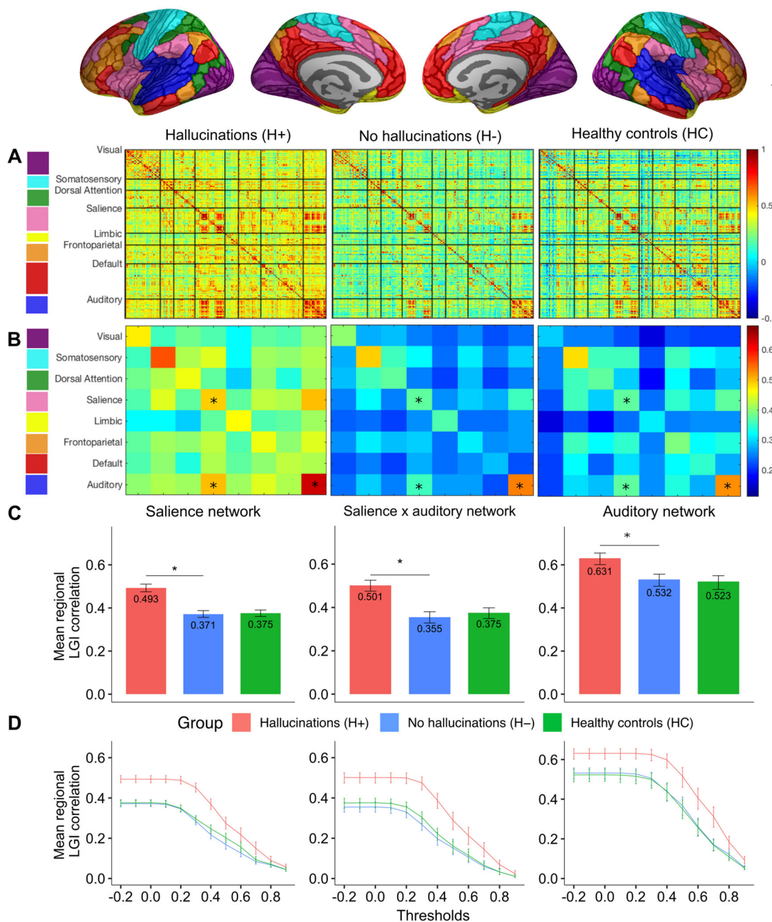
Fig. 4 Stages in construction and analysis of gyrification-based correlation matrices. A Local gyrification index (LGI) was computed for 360 parcellated brain regions (180 per hemisphere) according to the HCP-MMP1.0 atlas and was used to construct interregional Pearson's correlation ( 360 \times 360 ), adjusted for age, gender, scanning site, and intracranial volume for each of the three study groups (H+, H-, HC). Matrices were re-ordered according to eight well-established and replicable resting-state networks. B Each brain region was assigned a corresponding network and the LGI values between regions located within the same network were averaged, resulting in 8 \times 8 group-wise matrices. C Nonparametric permutation testing with 5000 resamplings was employed to test the significance of differences in patients with and without hallucinations in the mean LGI covariance within, and between, the salience and auditory networks. The observed differences in means were evaluated against the permutation null-distributions, and a two-tailed p -value calculated based on its percentile position (significance < 5\% ). D Mean regional LGI partial correlation within brain regions corresponding to the salience, salience-auditory interaction, and auditory networks for correlation thresholds ranging from -0.2 to 1 . Error bars represent the 95% bootstrap confidence intervals generated by resampling 5000 times with replacement across participants within each group. *FDR < 0.05 .
