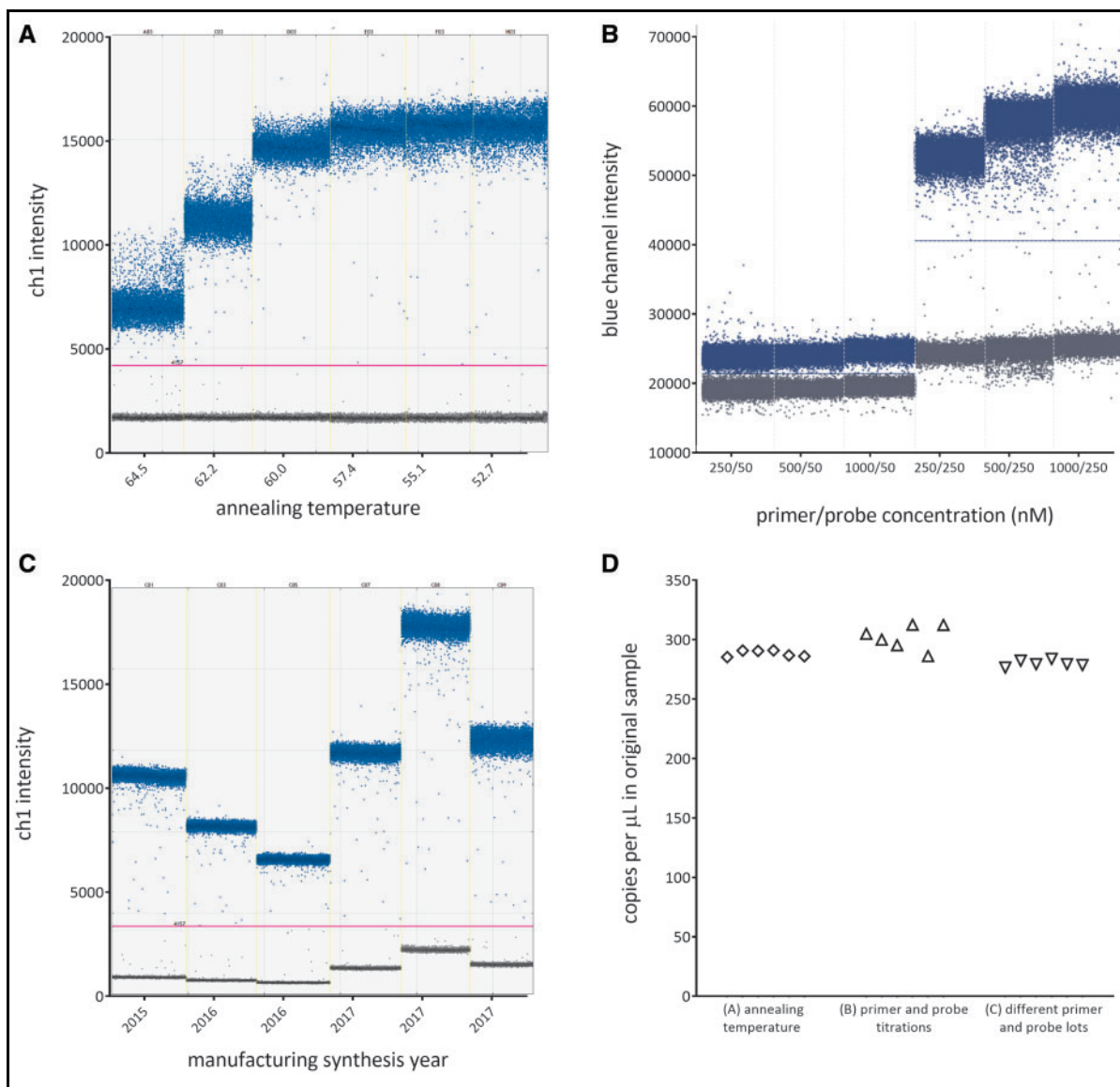
Fig. 2. Examples of the one color plot outputs demonstrating methodological robustness. The same assay and genomic DNA template is used in all parts of the figure. Unless otherwise stated, each reaction contains 900nM of each primer and 250nM of probe, annealing temperature: 60C, run for 40 PCR cycles. (A) The effect of the annealing temperature (gradient 65C to 52C from left to right) on the final fluorescence intensity of the positive and negative partitions. Each reaction contains approximately 20000 copies of the gDNA template analyzed using the QX200 (Bio-Rad) with Supermix for probes (no dUTP) (Bio-Rad). The horizontal pink line represents the threshold to separate the positive and negative partitions. (B) The effect of primer and probe concentrations on the difference in fluorescence intensity between positive and negative partitions. Reactions 1-3 have 250, 500, and 1000nM of primer, respectively, all with 50nM of probe. Reactions 4-6 have 250, 500, and 1000nM of primer, respectively all with 250nM of probe. Each reaction contains approximately 40000 copies of the gDNA template analyzed using the Naica (Stilla) and Perfecta Multiplex qPCR Toughmix (Quanta BioSciences). The blue horizontal lines represent the threshold to separate the positive and negative partitions. (C) The difference in fluorescence intensity of positive and negative partitions between 6 different batches of the same assay purchased between 2012 and 2017 from 3 different manufacturers. The genomic DNA template concentration and dPCR platform is the same as that described in (A). (D) Comparison of the copy number concentrations calculated from each of the 18 reactions shown in (A)-(C). Each reaction is represented by a symbol in the order it appears in its respective color plot.
