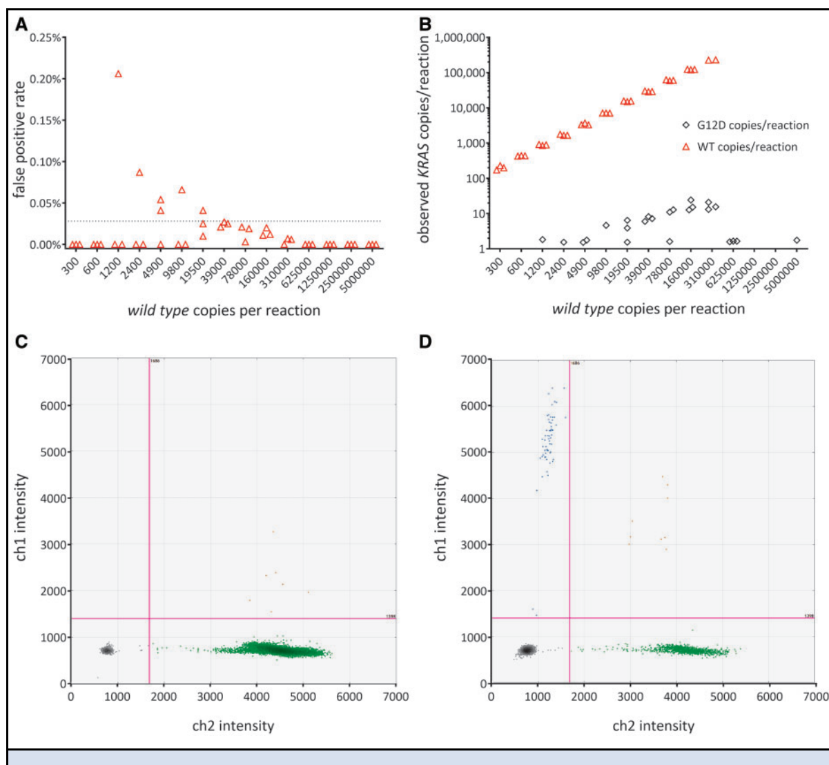
Fig. 4. An example of false positive rate of a single nucleotide variant assay. Example of the KRAS G12D mutation using the PrimePCR dPCR assay (Bio-Rad) and Supermix for probes (no dUTP) (Bio-Rad) using the QX200 (Bio-Rad) as described in (38). All reactions were performed in triplicate within a single experiment. (A) A 15-point two-fold serial dilution series from \sim 300 to \sim 5 million copies of the linearized KRAS wt plasmid was analyzed for G12D variant false signal to determine the false positive rate (FPR) over the wt dynamic range. FPR is linked to wt concentration with too few ( < 1200 ) or too many wt molecules ( > 625\,000 ) per reaction reducing the visible FPR. The horizontal dashed line represents the published FPR for this assay (38) that is quantifiable between 12 000 to 100 000 wt copies per reaction. (B) The corresponding copy number counts for the KRAS wt and G12D variant are shown. This demonstrates linearity in the wt measurements over the dynamic range (with quantities > 60\,000 being affected by saturation), and false G12D measurements associated with wt concentration. Examples of the two-color plots from the experiment of (C) a single well for the 39 000 wt copies/reaction showing the location of the false positive G12D partitions (orange) with the negative (grey) and wt only (green) clusters and (D) a positive control reaction using the 5% allelic frequency of the Multiplex I cfDNA Reference Standard Set (Horizon Discovery) to show the location of the single positive G12D cluster (blue). The pink lines represent the threshold to separate the positive and negative partitions and are at the same fluorescence intensity for C and D.
