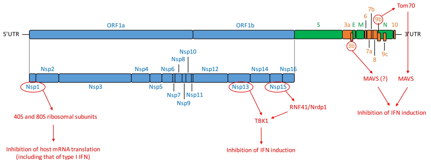
Fig 1. SARS-CoV-2 genomic organization and encoded proteins. ORF1a/b encode a polyprotein, which is proteolytically processed into Nsp1–16, represented in blue. Structural proteins, including S, E, M, and N proteins are in green. Accessory proteins encoded at the 3' end of the viral genome comprise ORF3a, 3b, 6, 7a, 7b, 8, 9b, 9c, and 10 and are colored in orange. Untranslated extremities of the genome (5'-UTR and 3'-UTR) are also represented. In red are depicted SARS-CoV-2 proteins that interfere with IFN induction pathway as well as their known or hypothetical target [5, 37, 147]. E, envelope; IFN, interferon; M, membrane; MAVS, mitochondrial antiviral-signaling protein; N, nucleocapsid; Nrdp1, neuregulin receptor degradation protein-1; Nsp, nonstructural protein; ORF, open reading frame; RNF41, ring finger protein 41; S, spike; SARS-CoV-2, severe acute respiratory syndrome coronavirus-2; TANK, TRAF family member-associated NF-κB activator; TBK1, TANK-binding kinase 1; Tom70, translocase of outer mitochondrial membrane 70; UTR, untranslated region.
