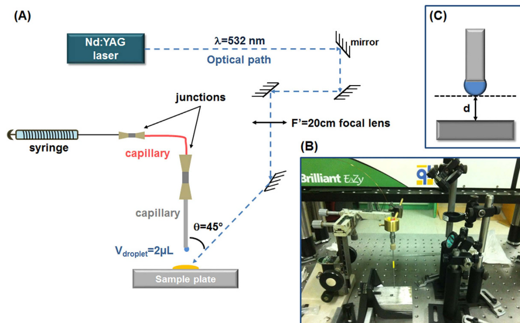
Figure 9. (A) Schematic representation and (B) photograph of the LADC experimental setup. The measurement of the height between the droplet and the sample is schematized in (C).
