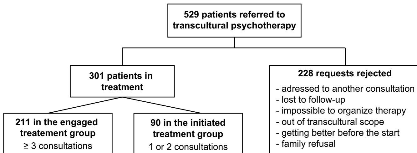
Fig 1. Study flowchart.
